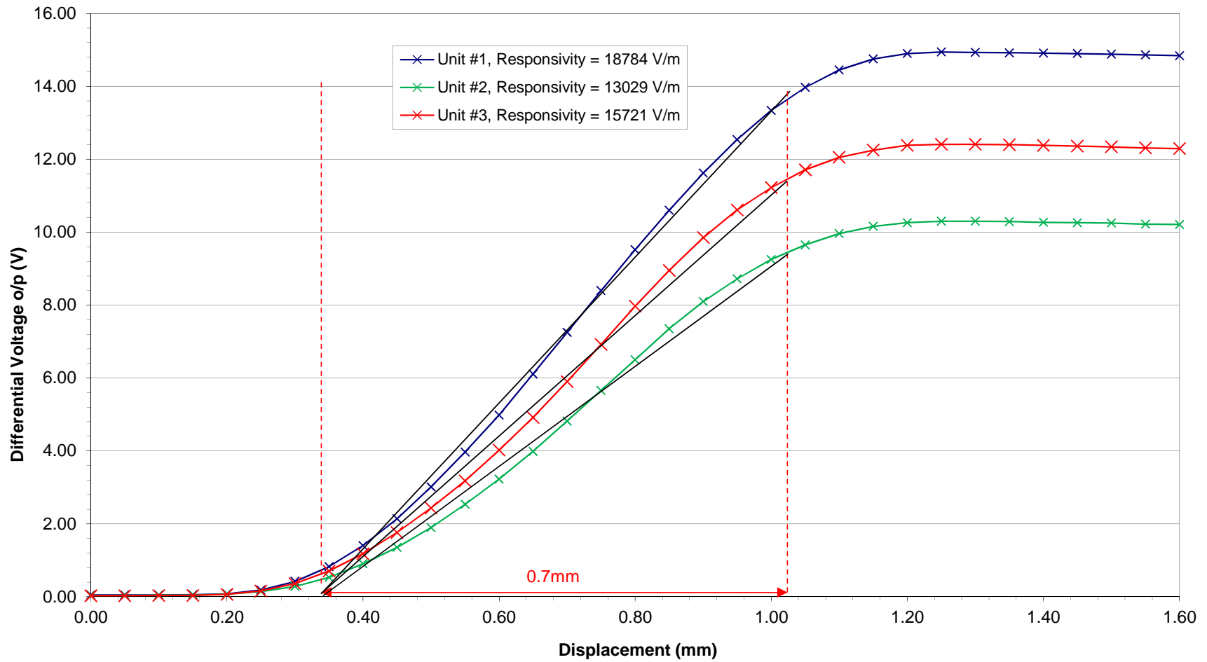
AOSEM Characterisation - Responsivity Plot (Differential Output)
