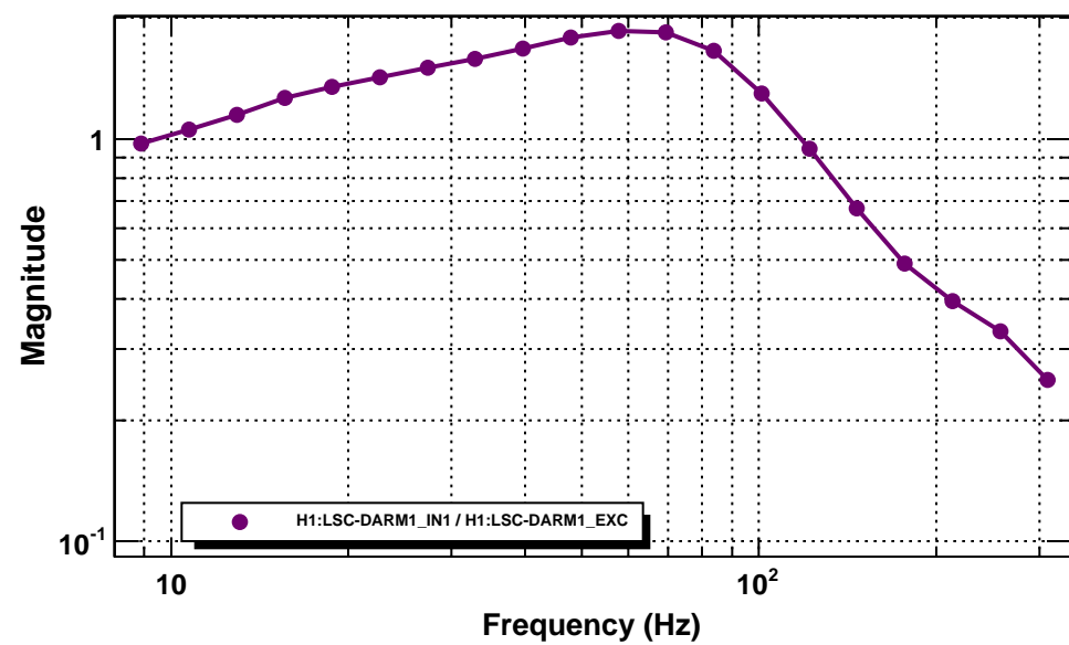
Transfer function
