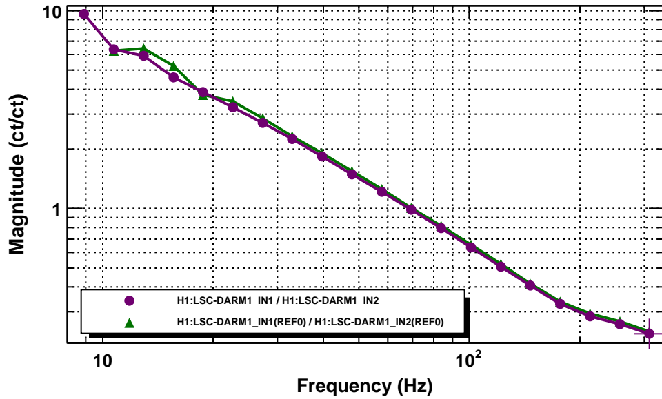
Transfer function
