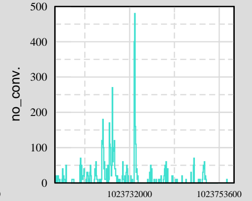
Ch 12: H0:PEM-LAB_DST2_5
