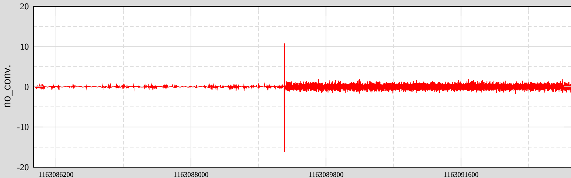
Ch 1: H1:PSL-FSS_FAST_MON_OUTPUT
