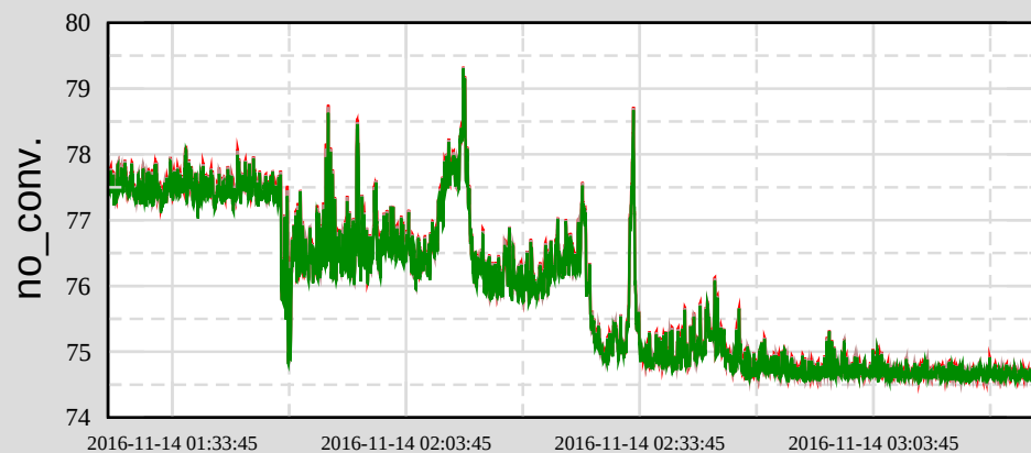
Ch 6: H1:PSL-PWR_PMC_SUM
