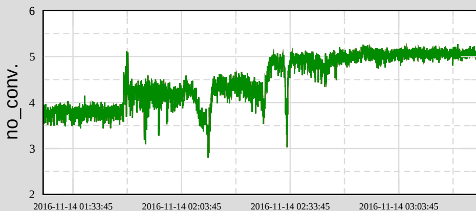
Ch 1: H1:PSL-ISS_DIFFRACTION_AVG
