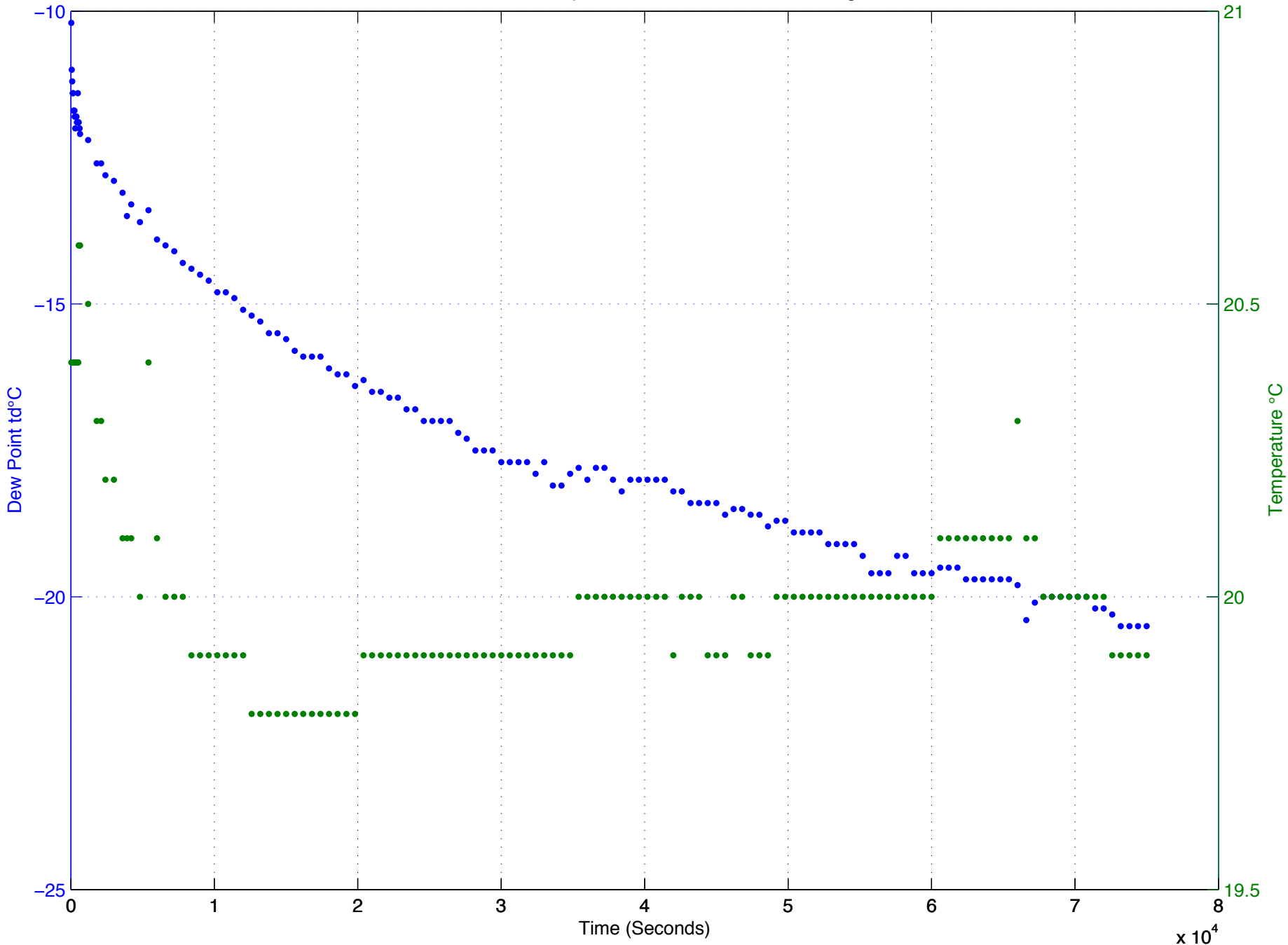
Dew Point & Temperature for HAM6 Container Purge
