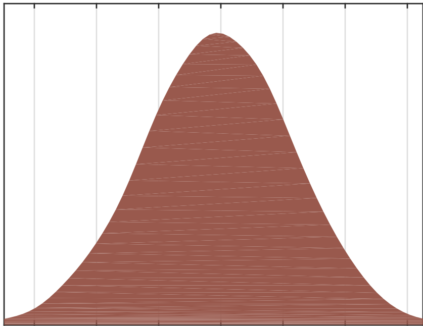
H1SUSEMY_L1 act. coef. covariance (MCMC)
