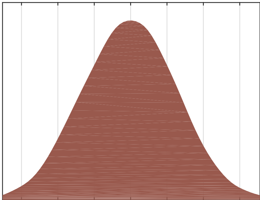
H1SUSEMY_L2 act. coef. covariance (MCMC)
