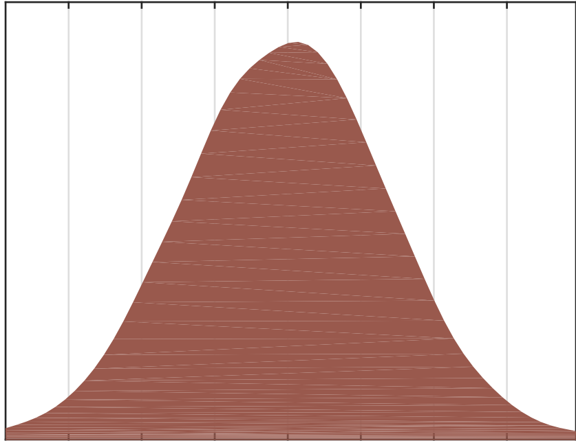
H1SUSEMY_L3 act. coef. covariance (MCMC)
