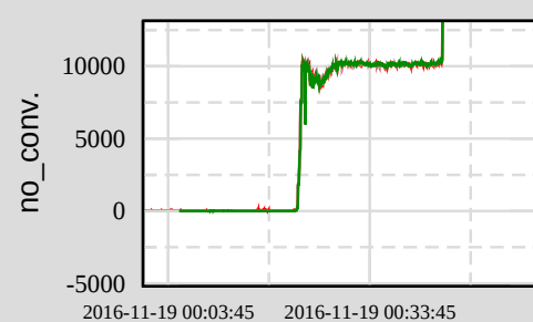
Ch 9: H1:LSC-X_TIDAL_REDTRIG_INMON
