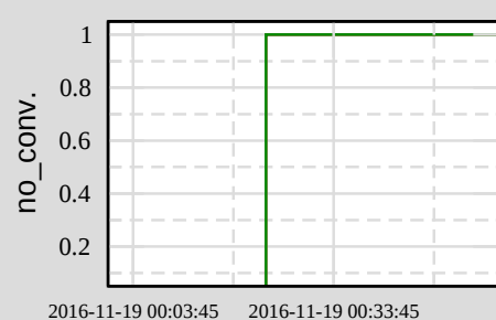
Ch 11: H1:LSC-X_TIDAL_STATE
