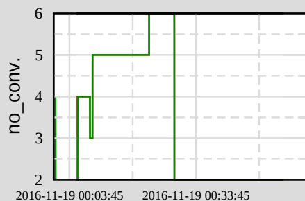
Ch 3: H1:ALS-C_LOCK_REQUESTY
