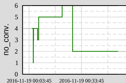
Ch 7: H1:LSC-Y_TIDAL_REQUEST
