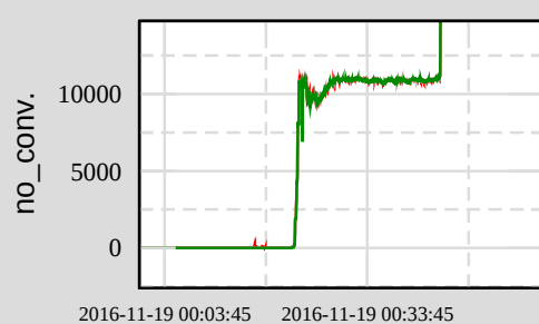
Ch 5: H1:LSC-Y_TIDAL_REDTRIG_INMON
