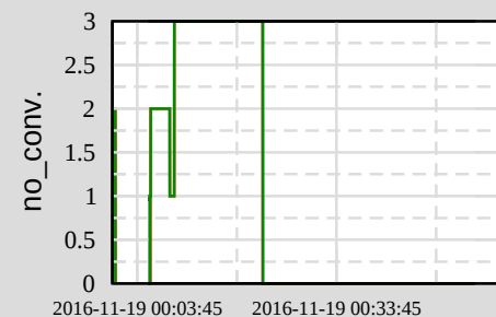
Ch 15: H1:LSC-Y_TIDAL_CTRL_OUT16
