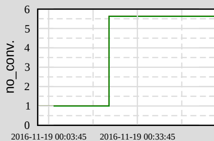
Ch 1: H1:ASC-Y_TR_B_NSUM_GAIN
