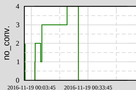
Ch 6: H1:LSC-Y_TIDAL_SEND
