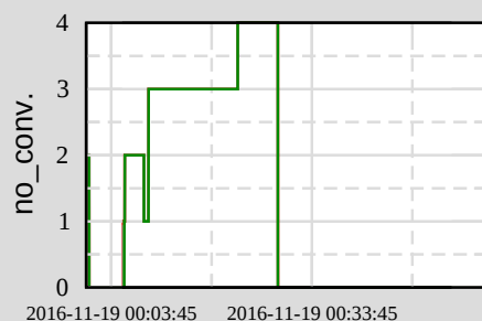
Ch 5: H1:LSC-Y_TIDAL_REDTRIG_INMON
