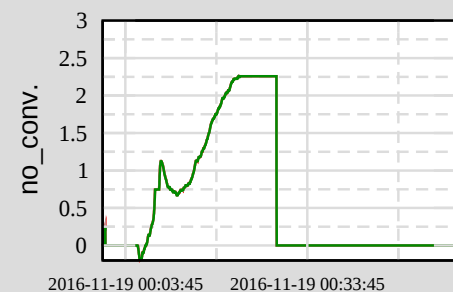
Ch 14: H1:LSC-X_TIDAL_CTRL_OUT16
