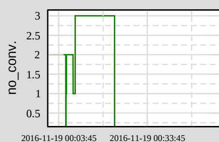
Ch 10: H1:LSC-X_TIDAL_REDTRIG_MON
