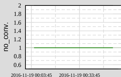
Ch 1: H1:ASC-Y_TR_B_NSUM_GAIN
