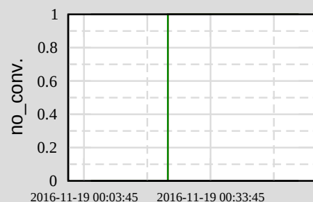
Ch 9: H1:LSC-X_TIDAL_REDTRIG_INMON
