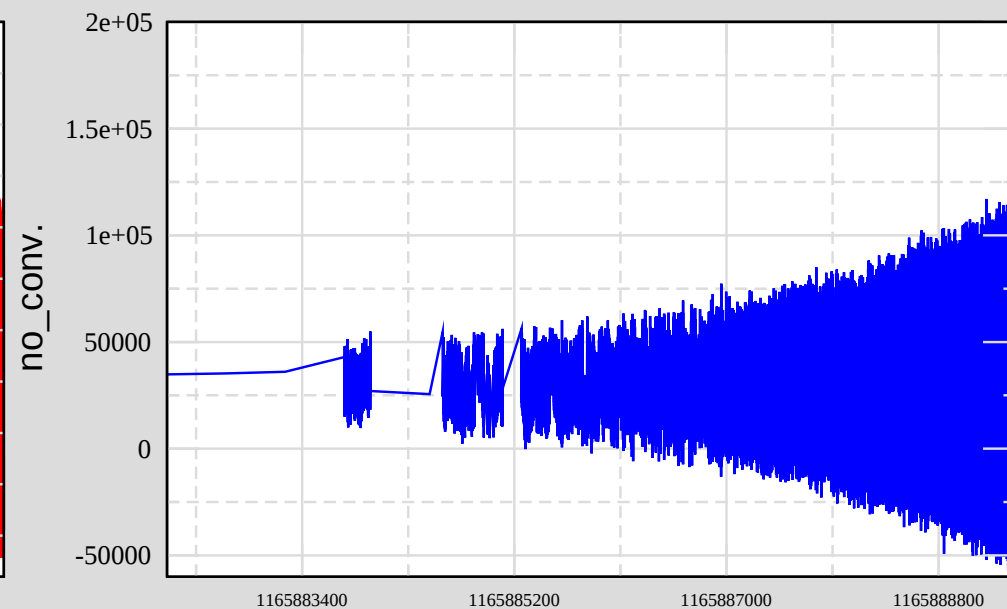
Ch 7: H1:SUS-ETMY_L3_ESDOUTF_UR_OUTPUT
