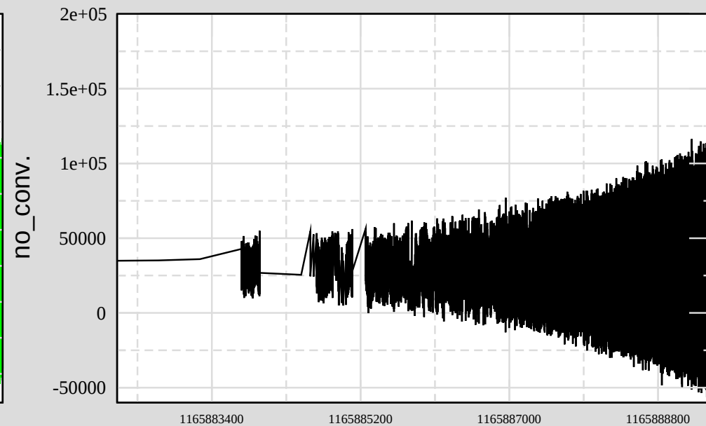
Ch 8: H1:SUS-ETMY_L3_ESDOUTF_LR_OUTPUT
