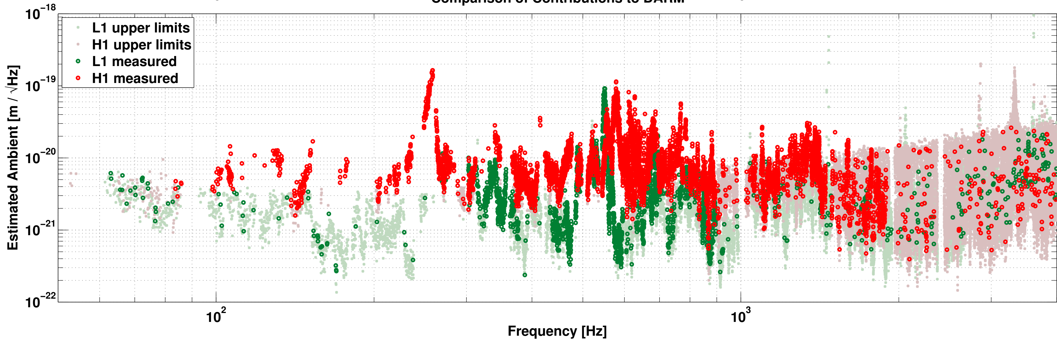
Comparison of Contributions to DARM
