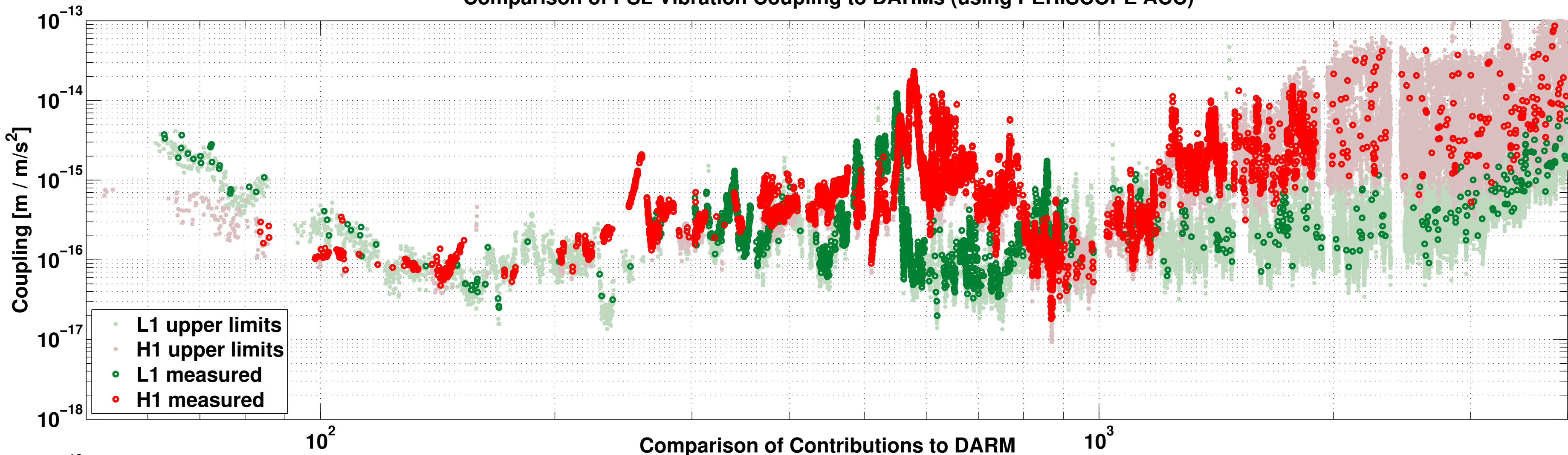
Comparison of PSL Vibration Coupling to DARMs (using PERISCOPE ACC)
