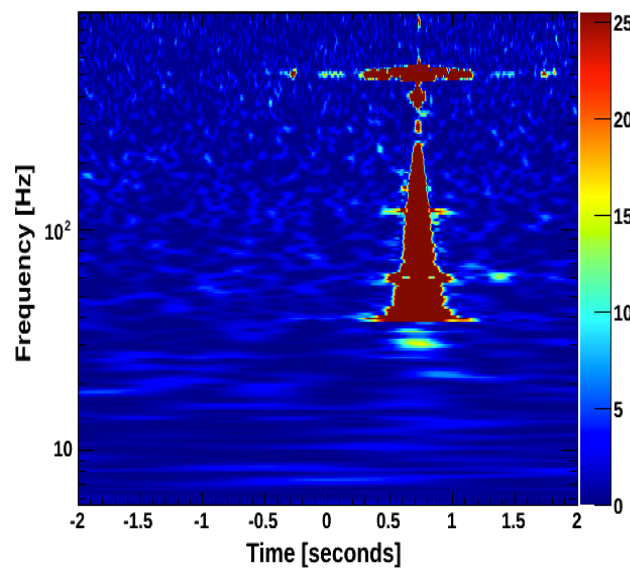
H1:SUS-ETMY_L2_NOISEMON_LR_OUT_DQ at 1166271159.000 with Q of 45.3
