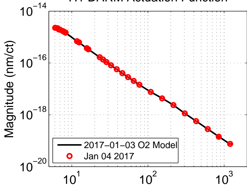
H1 DARM Actuation Function
