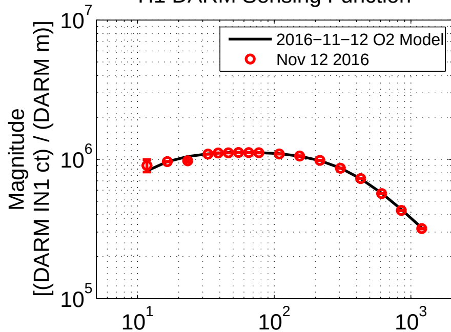
H1 DARM Sensing Function
