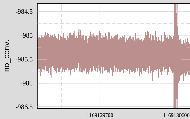
Ch 4: H1:SUS-ETMX_L2_WIT_YMON
