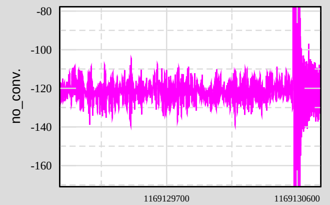
Ch 9: H1:SUS-ETMY_L2_WIT_PMON
