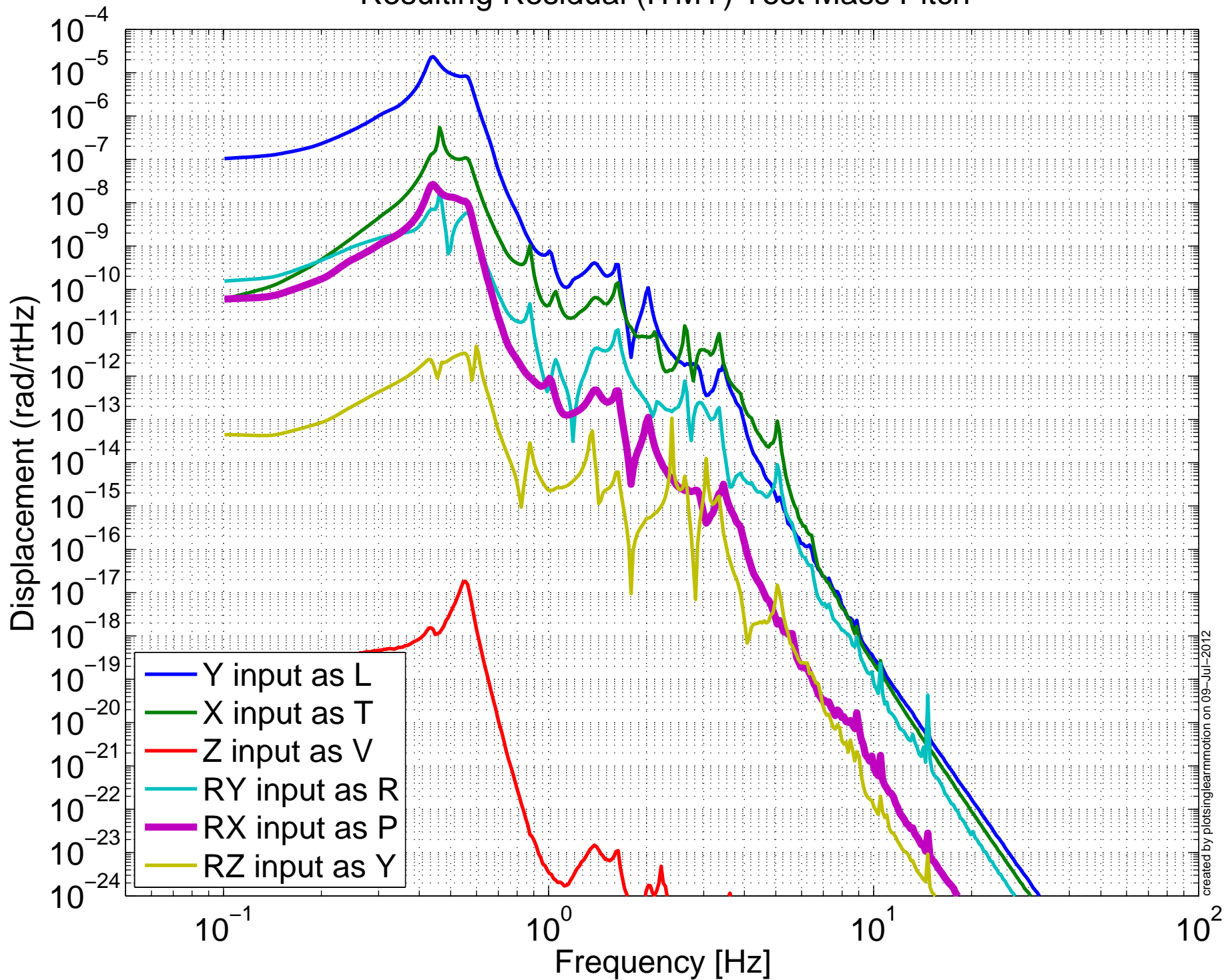
Resulting Residual (ITMY) Test Mass Pitch
