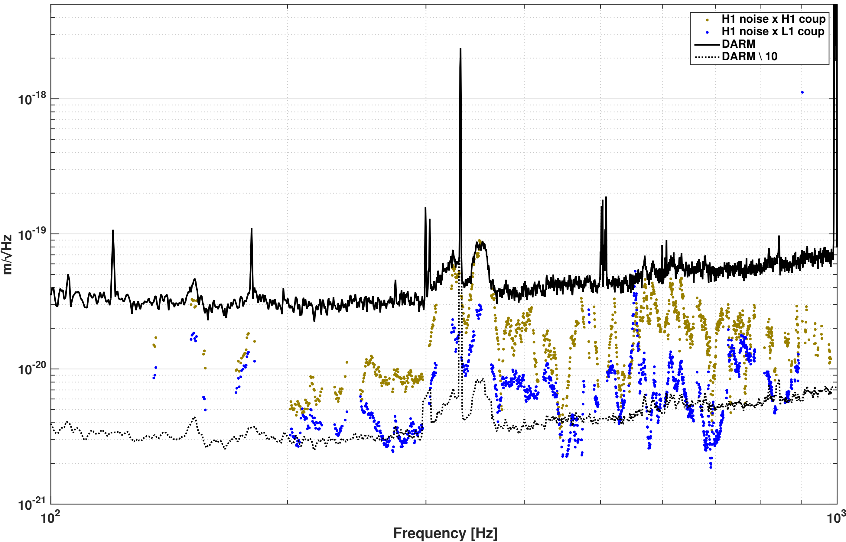
Contributions to H1 DARM, with WFS A DC, different couplings
