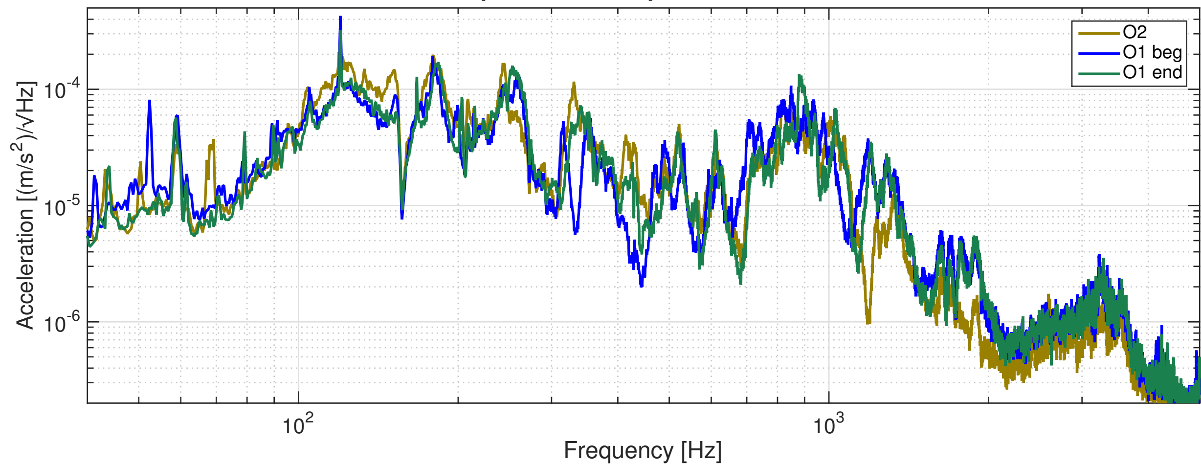
H1 Periscope motion comparison, Normal Ambient
