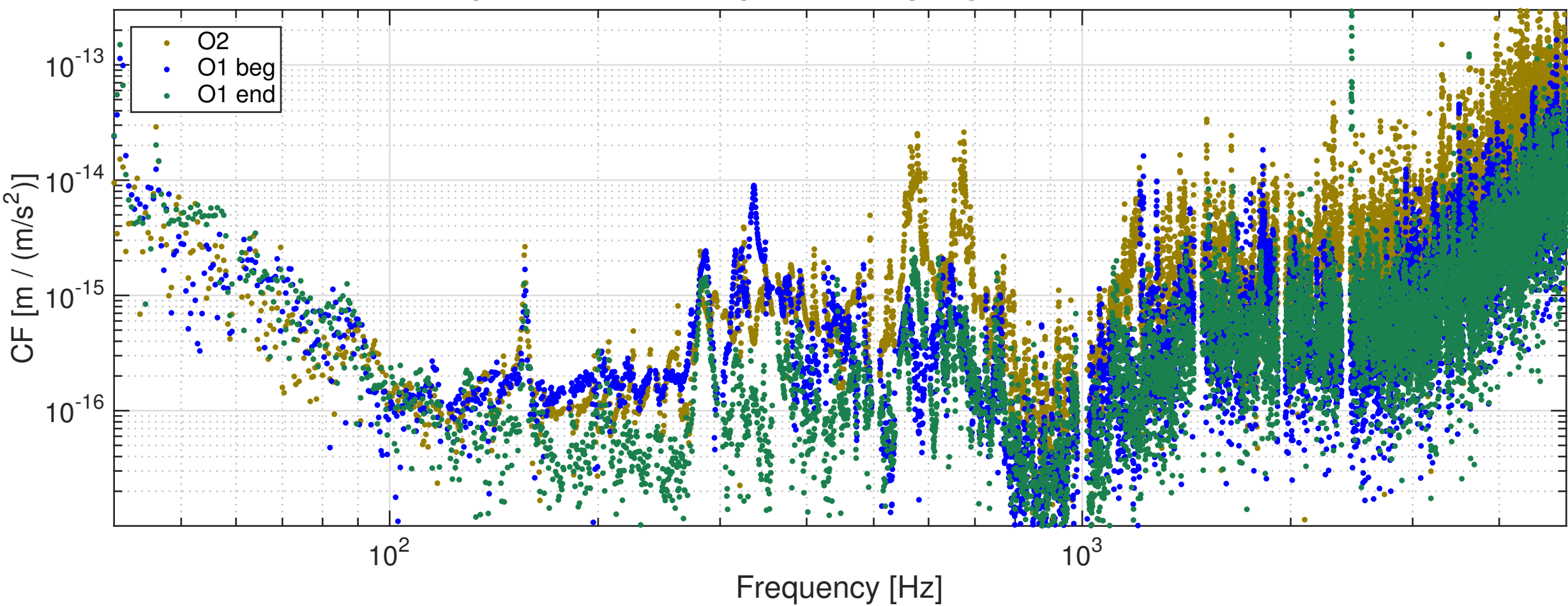
Comparison of Periscope Acc Coupling Functions to DARM
