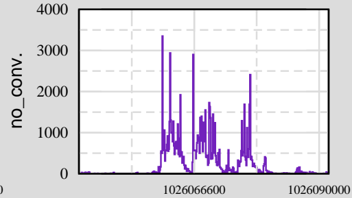
Ch 9: H0:PEM-EY_DST1_5
