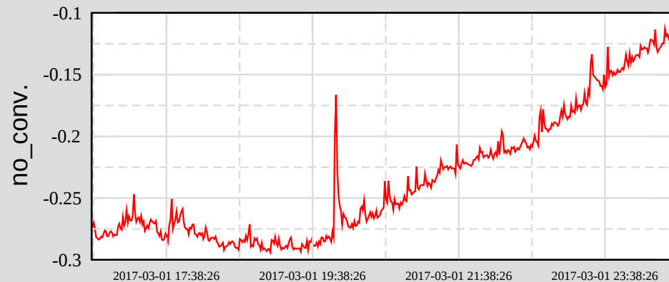
Ch 4: H0:VAC-MX_GV15_II329_AIP_IC_LOGMA
