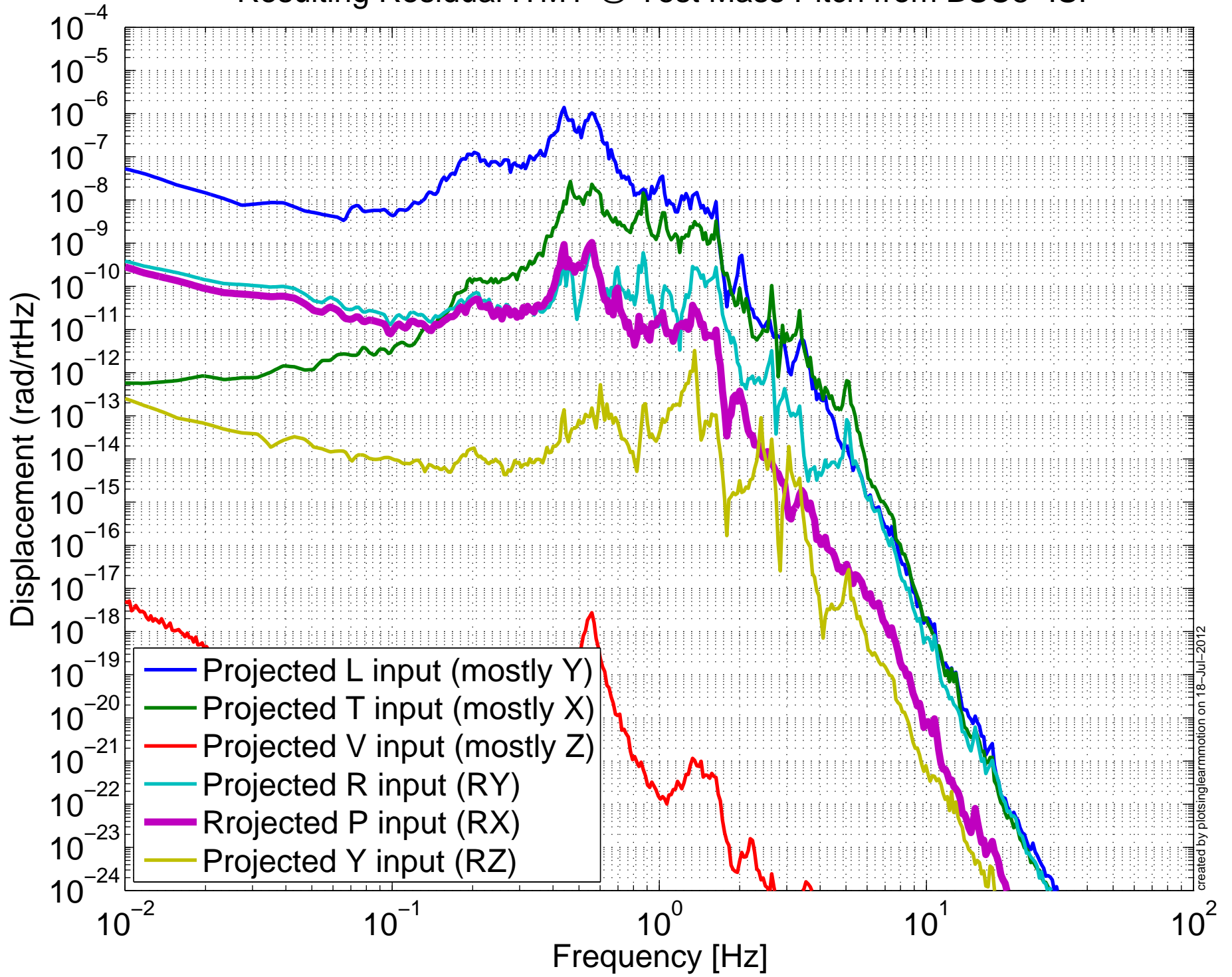
Resulting Residual ITMY @ Test Mass Pitch from BSC8-ISI
