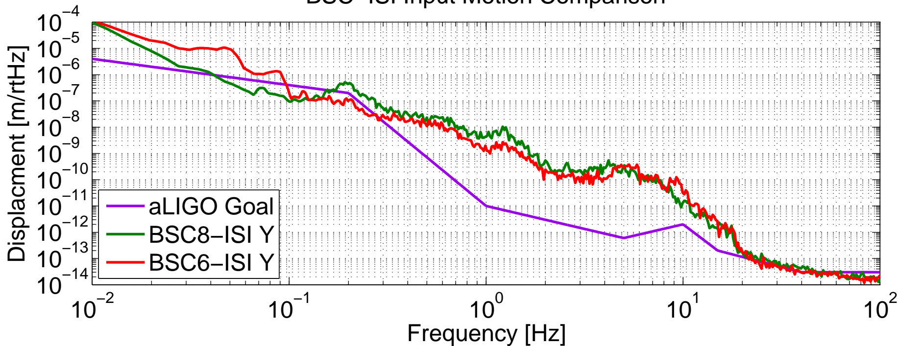
BSC-ISI Input Motion Comparison
