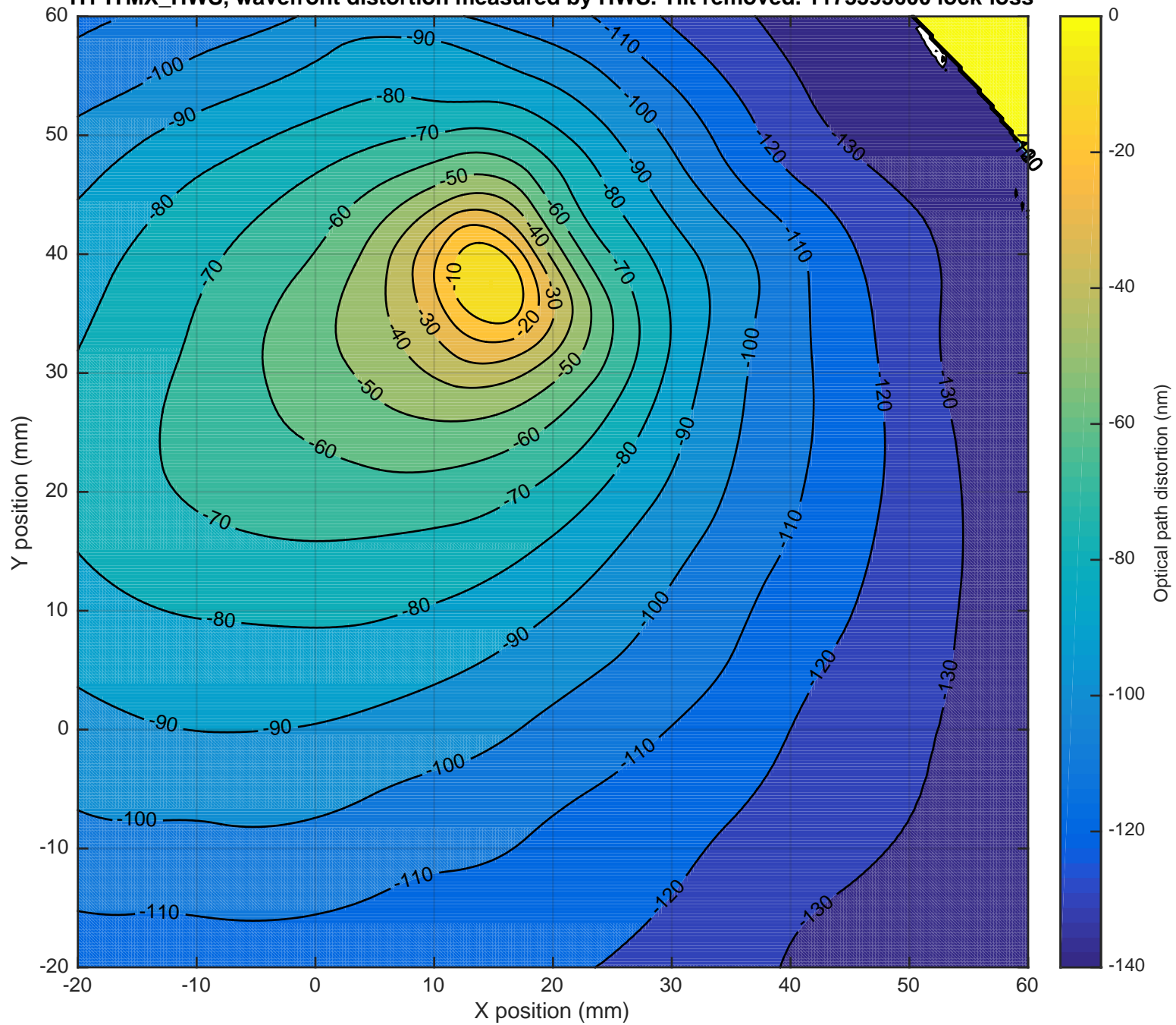
H1-ITMX_HWS, wavefront distortion measured by HWS. Tilt removed. 1173593600 lock-loss
