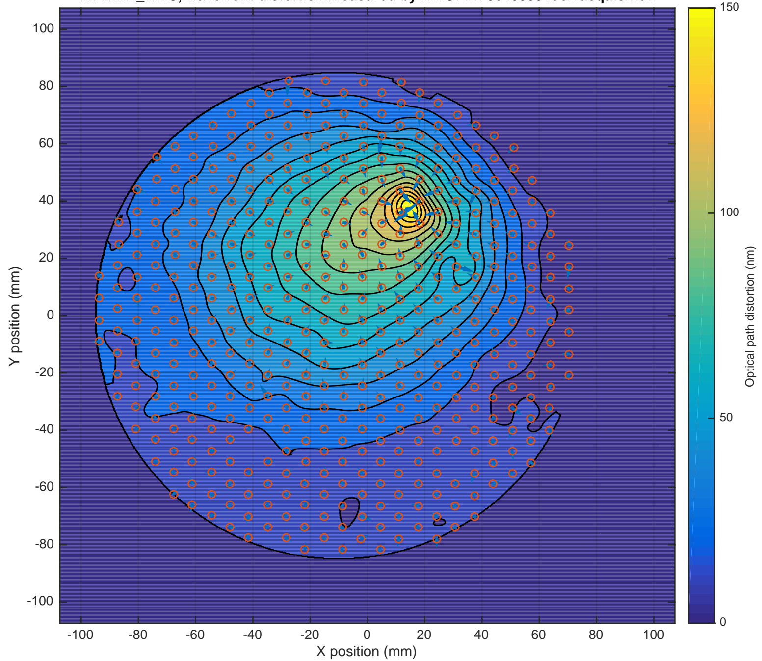
H1-ITMX_HWS, wavefront distortion measured by HWS. 1173640800 lock acquisition
