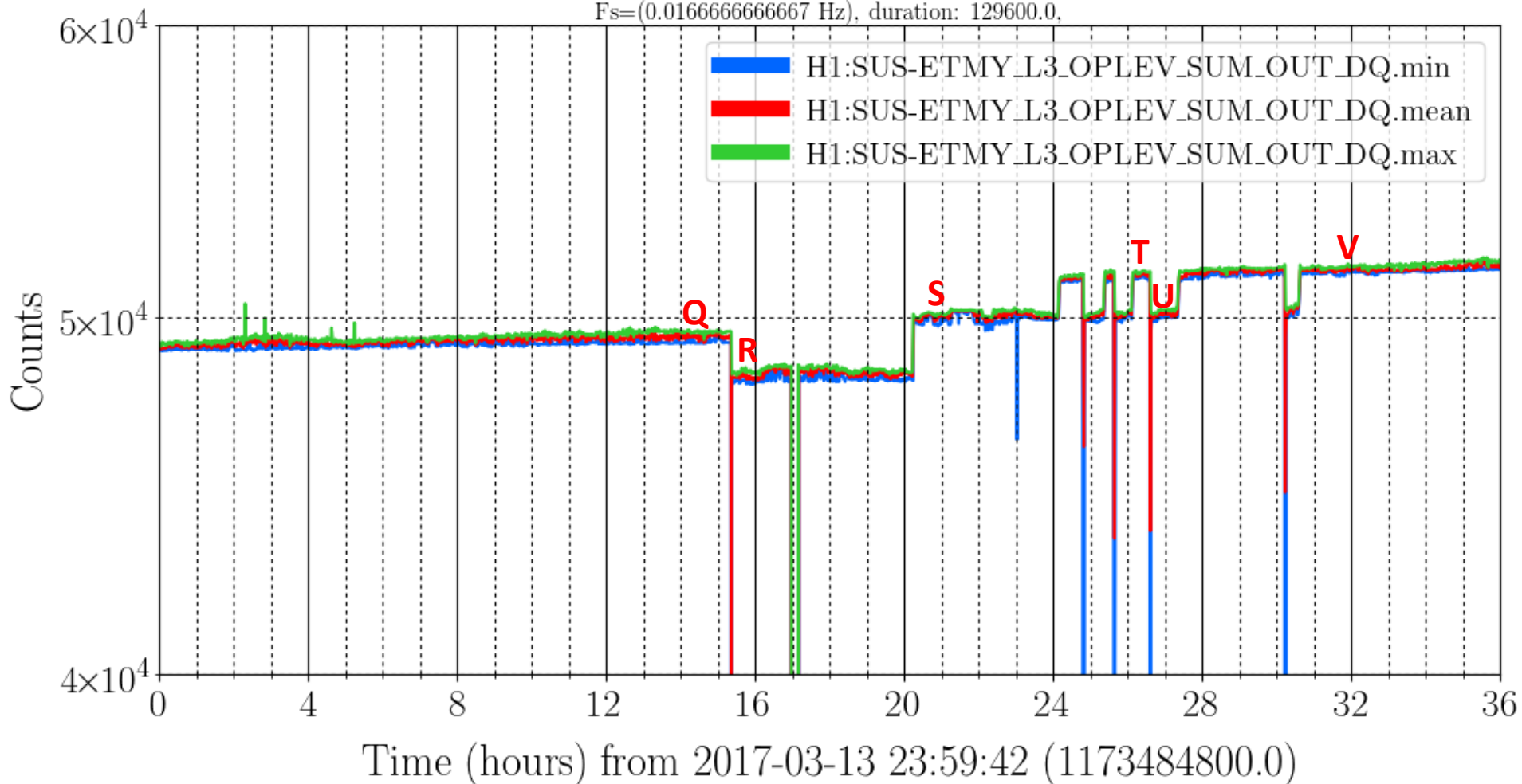
Time series: H1:SUS-ETMY_L3_OPLEV_SUM_OUT_DQ.min
