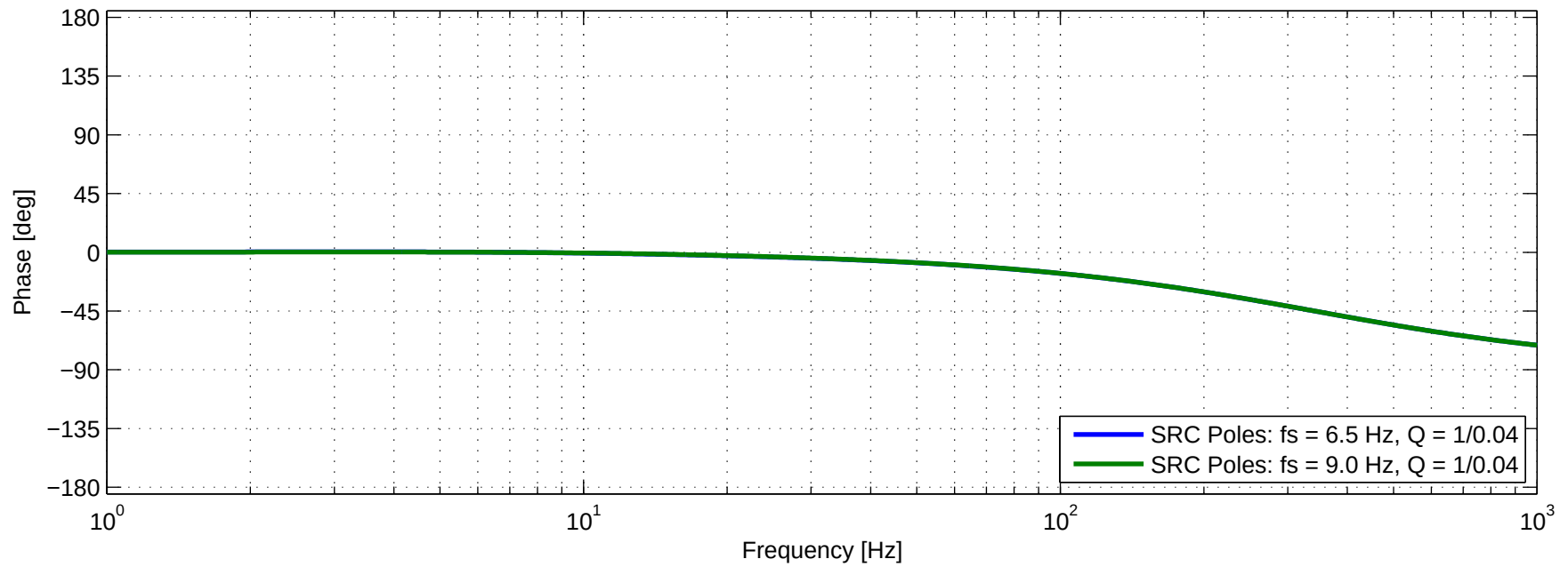
Example Extremes of SRC Detuning at H1 180/\pi \cdot \angle [ H_c \cdot (1 / 1 + i (f / f_c) ) \cdot (f^2 / (f^2 - i (f f_s / Q) + f_s^2) ) ]
