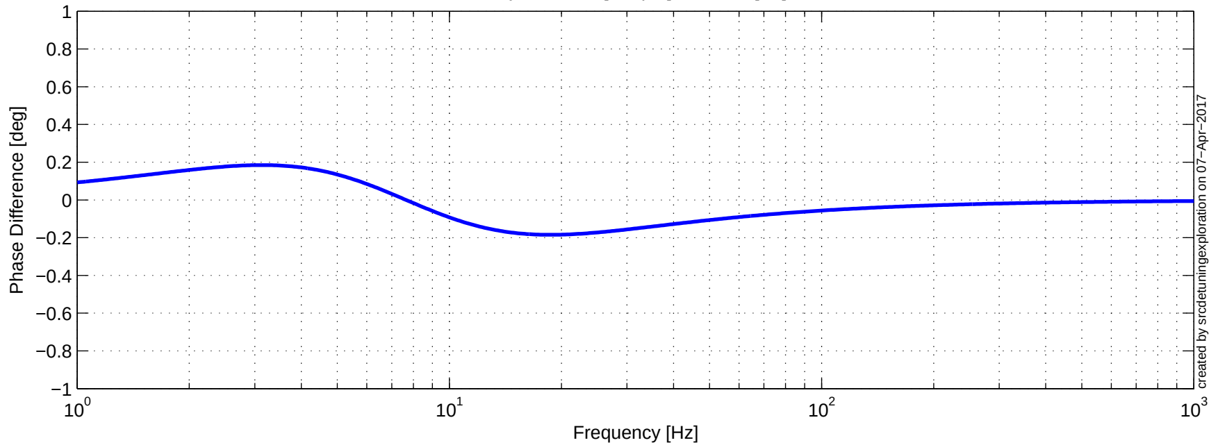
Toy: H_c = 3.6 [mA/pm], f_c = 341 [Hz]
