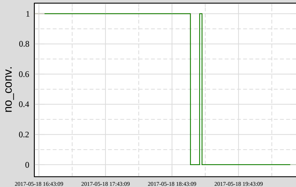
Ch 6: H0:VAC-EY_Y3_410_PWR_REQ
