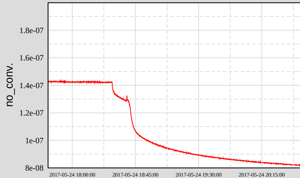
Ch 3: H0:VAC-LX_X2_PT170_MOD1_PRESS_TORR
