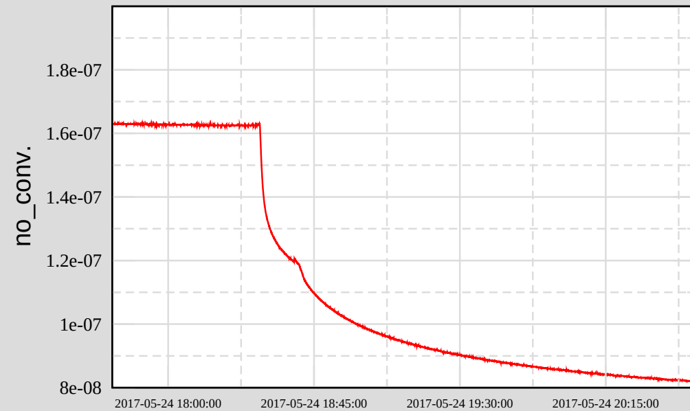
Ch 1: H0:VAC-LX_Y2_PT180_MOD1_PRESS_TORR
