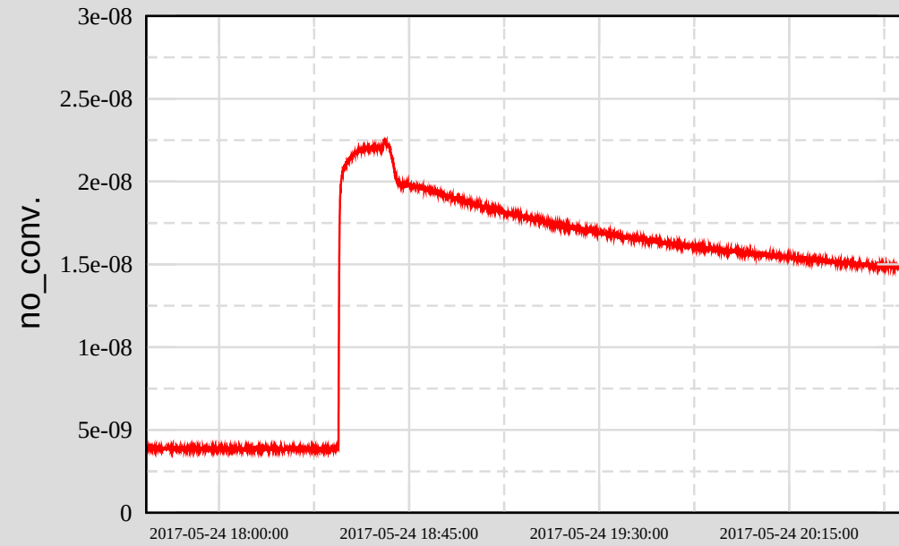
Ch 2: H0:VAC-LY_Y3_PT114B_PRESS_TORR
