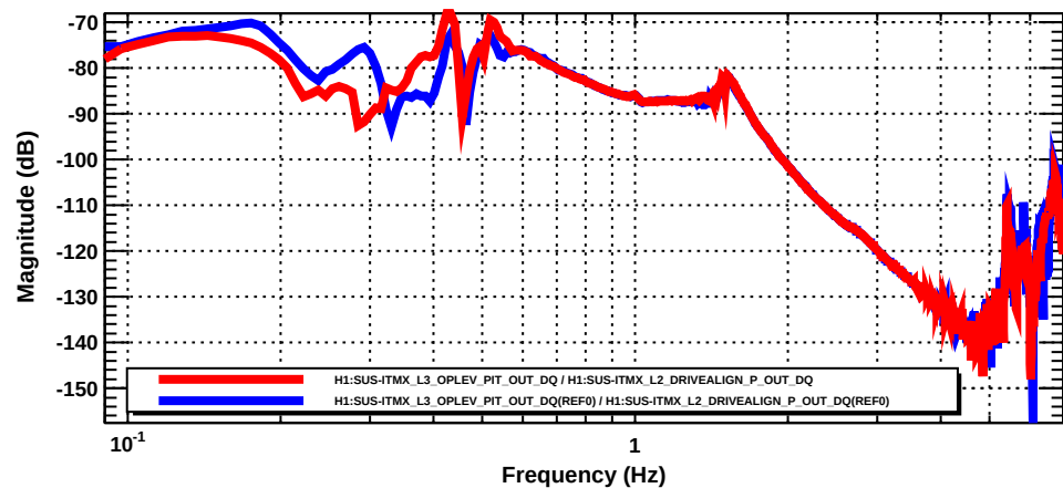
Transfer function
