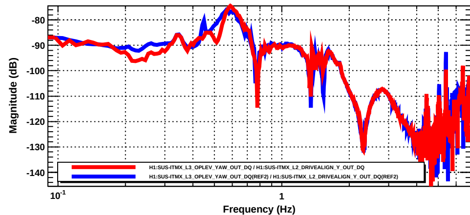
Transfer function
