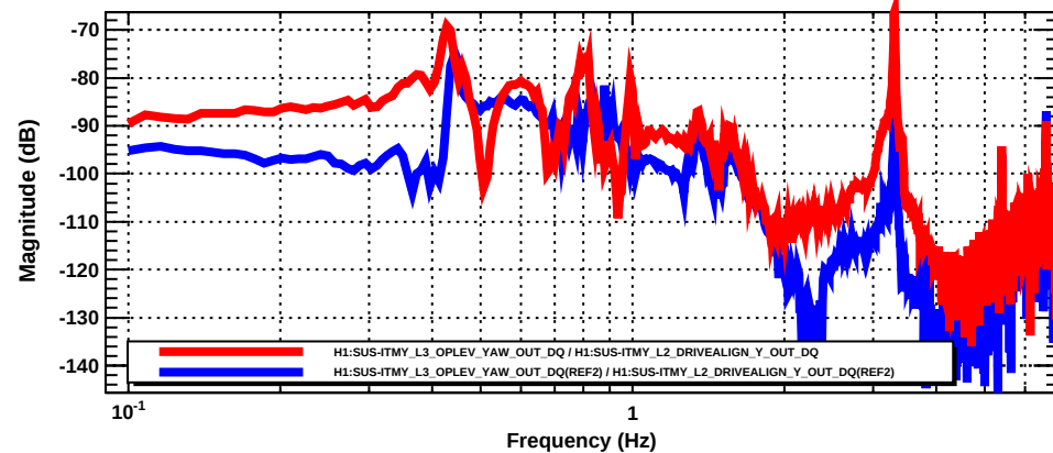
Transfer function
