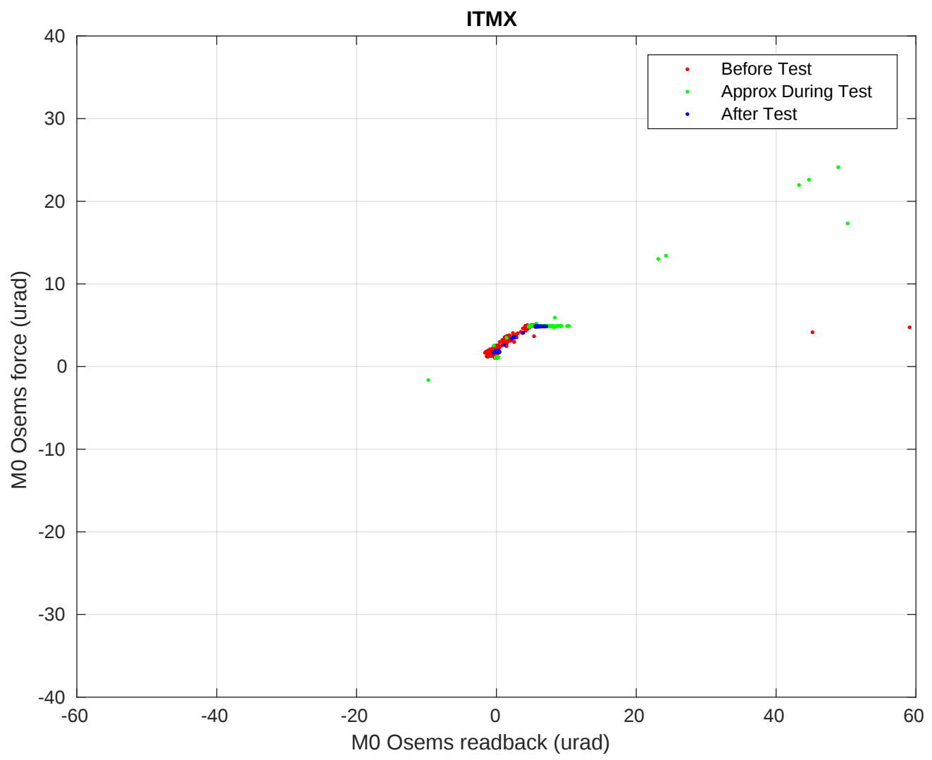
Linear relationship between top mass force and top mass position offset by EQ
