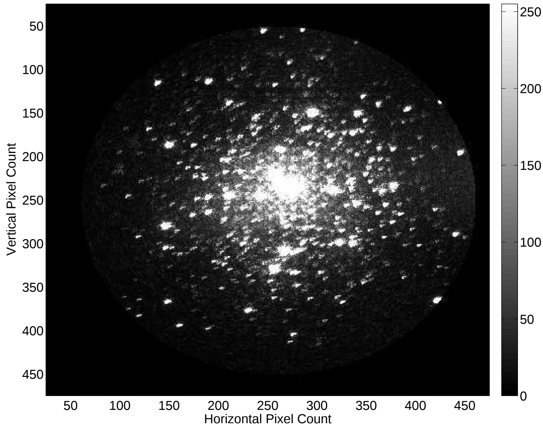
H1 ETMX Red Camera; DC Readout, 2W 2017-08-29 Pre-TMDS Discharge
