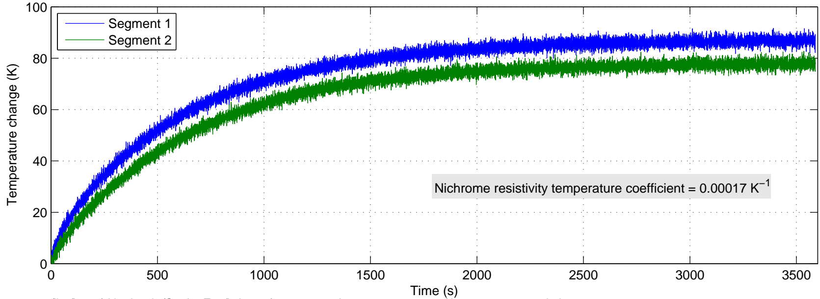
Ring heater temperature vs time – requested current = 630 mA
