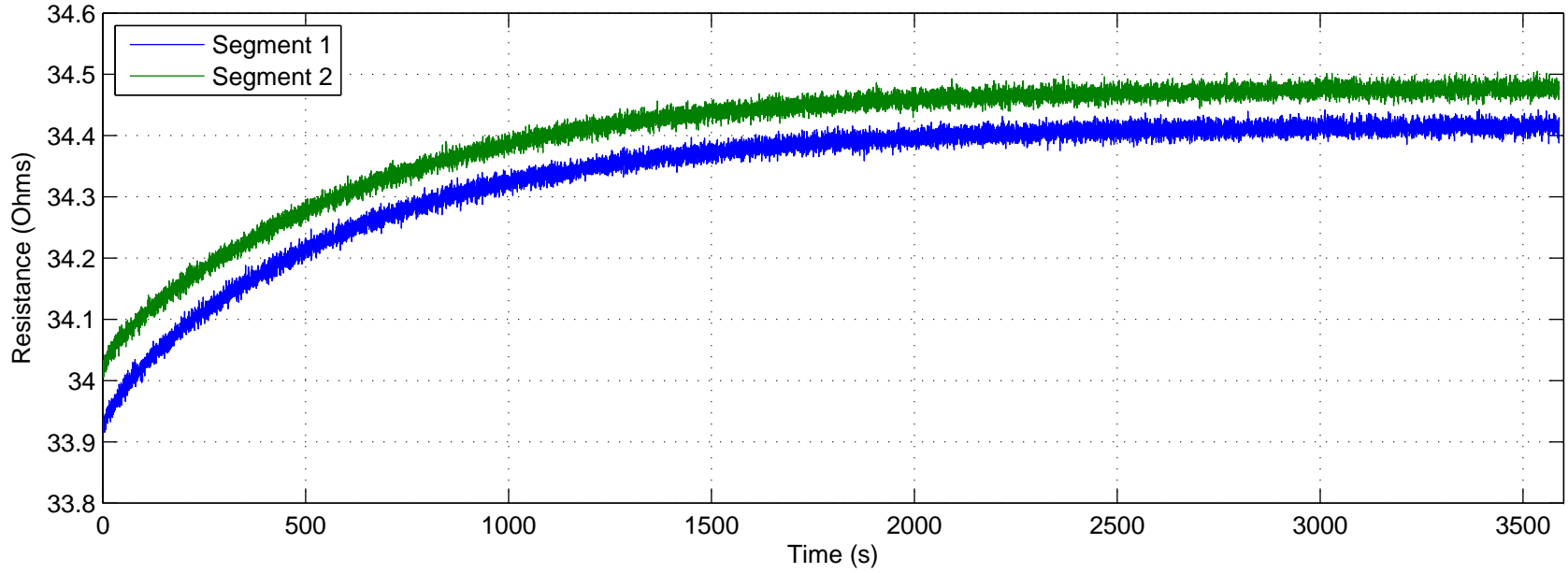
Ring heater resistance vs time – requested current = 630 mA
