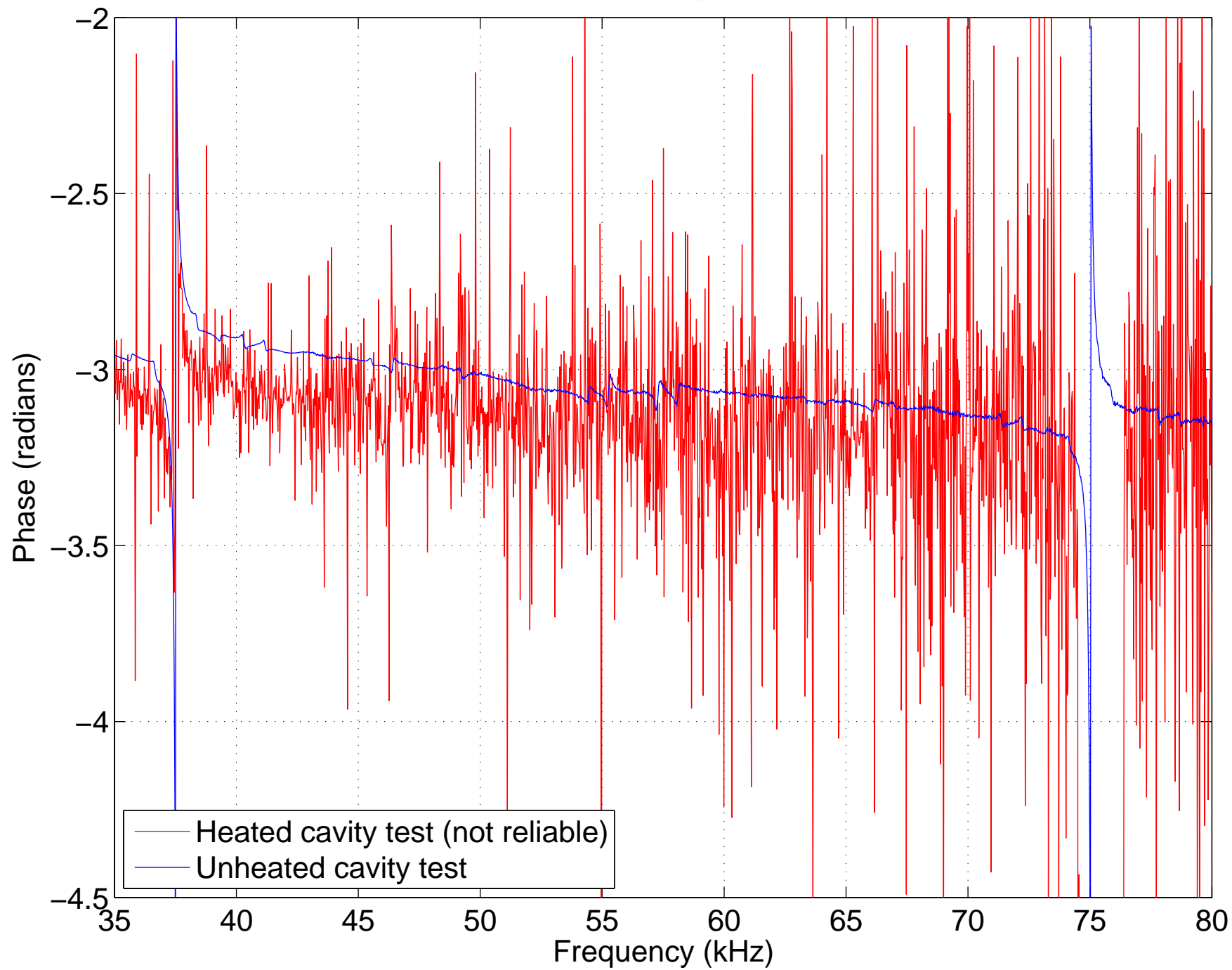
Phase response of the cavity to injected sidebands
