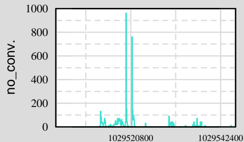
Ch 11: H0:PEM-LAB_DST1_5
