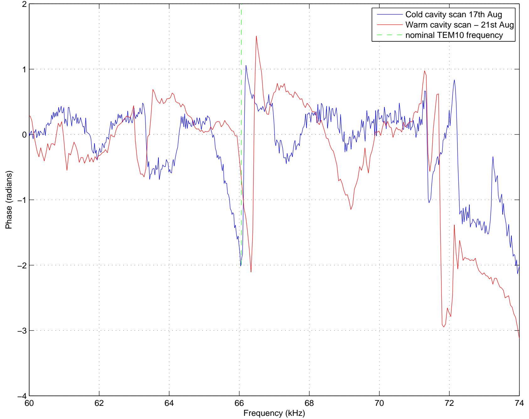
TEM10 location with cold and hot cavity scans
