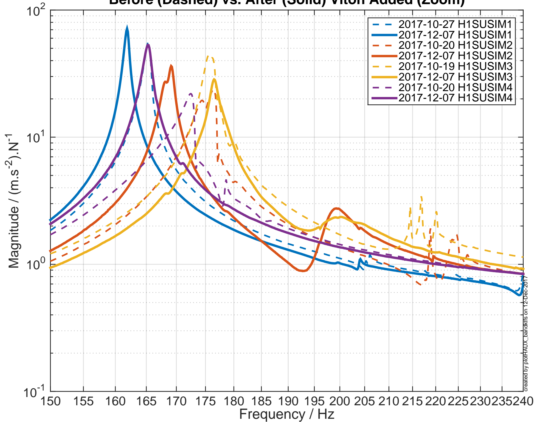
H1 HAUX Cage Resonance Comparison, All IMs, Longitudinal Before (Dashed) vs. After (Solid) Viton Added (Zoom)
