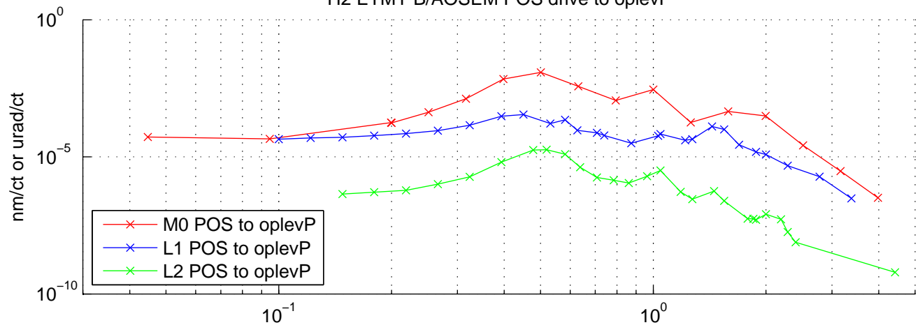
H2 ETMY B/AOSEM POS drive to oplevP
