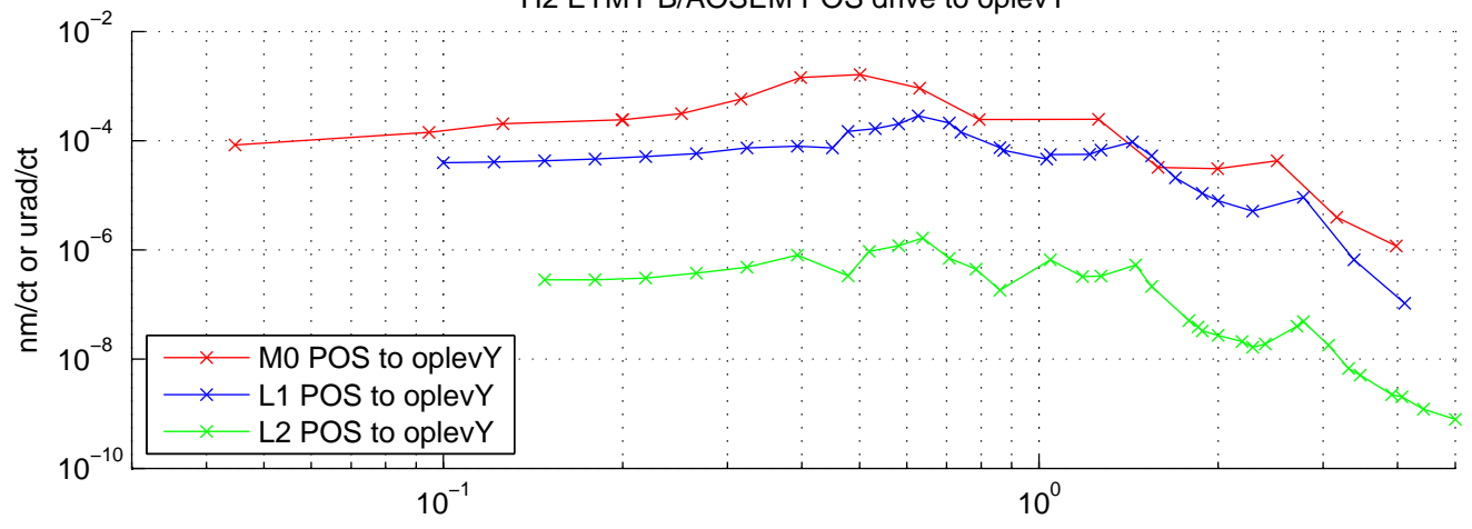
H2 ETMY B/AOSEM POS drive to oplevY
