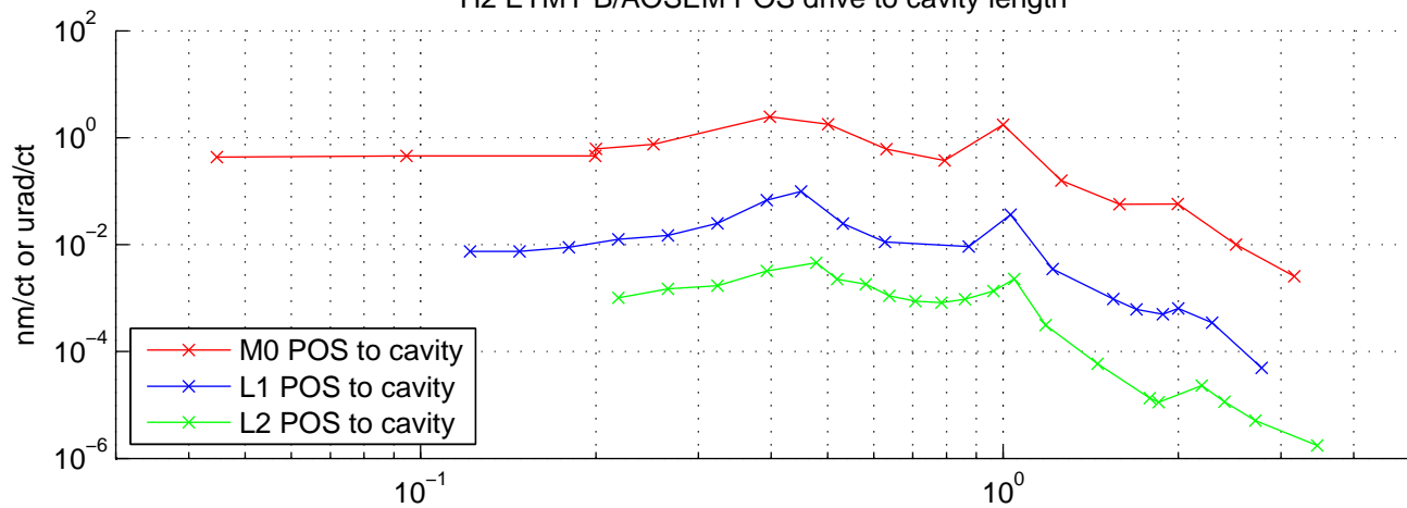
H2 ETMY B/AOSEM POS drive to cavity length
