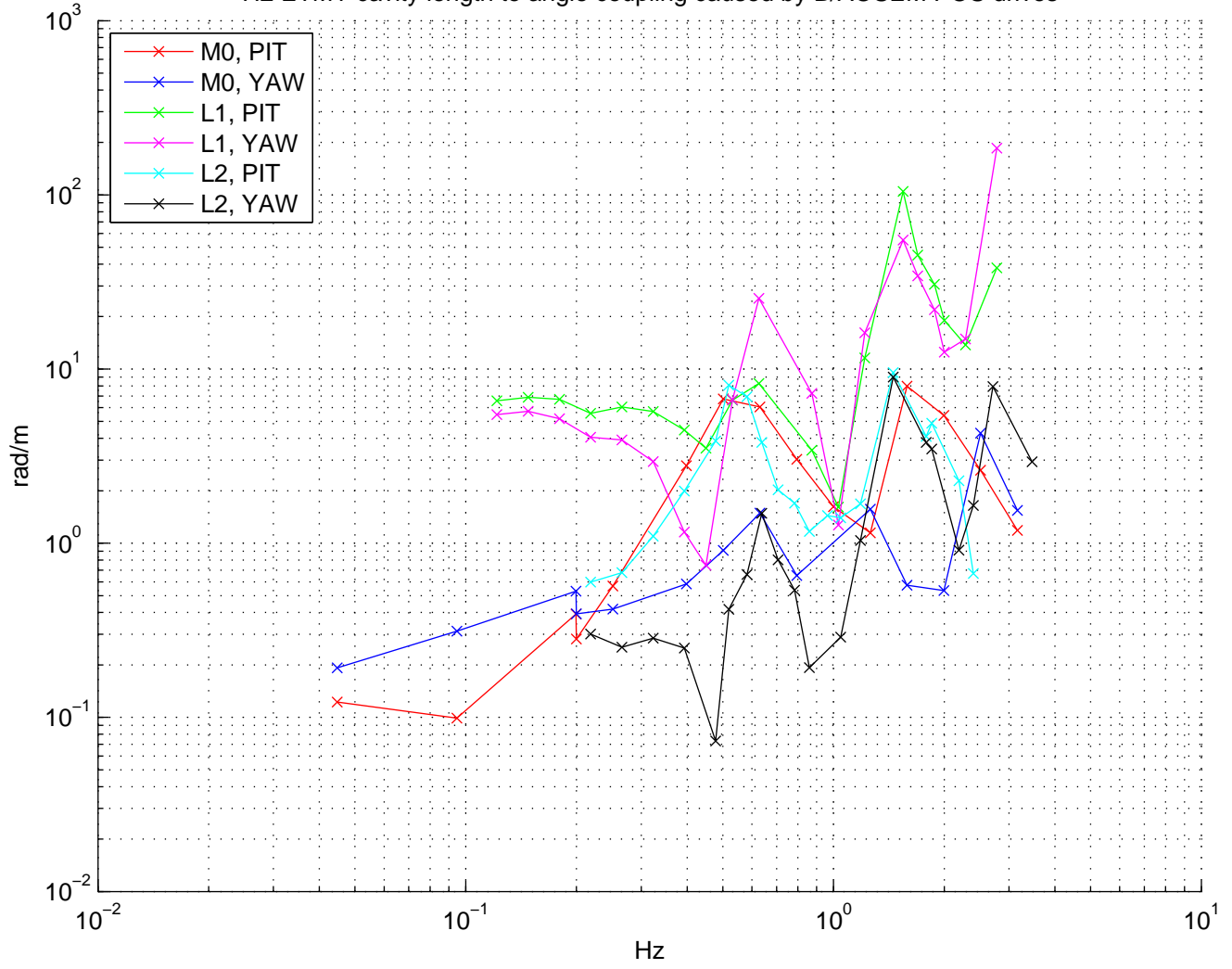
H2 ETMY cavity length to angle coupling caused by B/AOSEM POS drives
