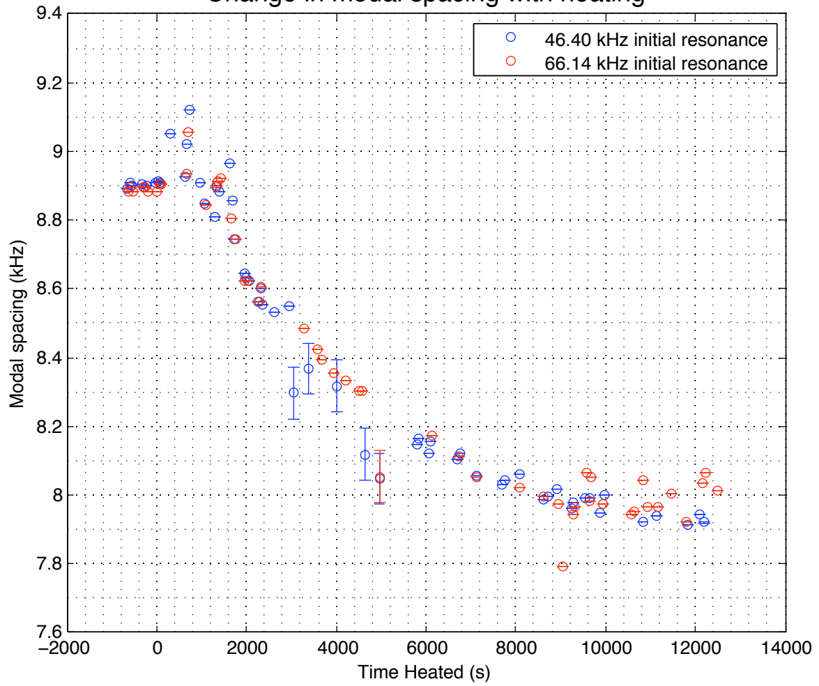
Change in modal spacing with heating
