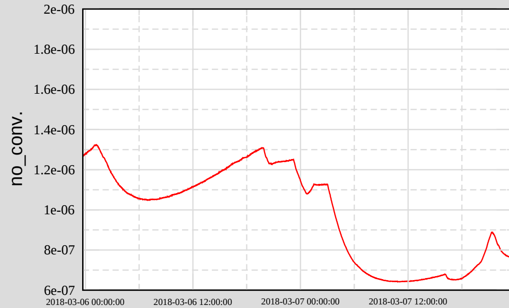
Ch 2: H0:VAC-MY_Y4_PT245B_PRESS_TORR
