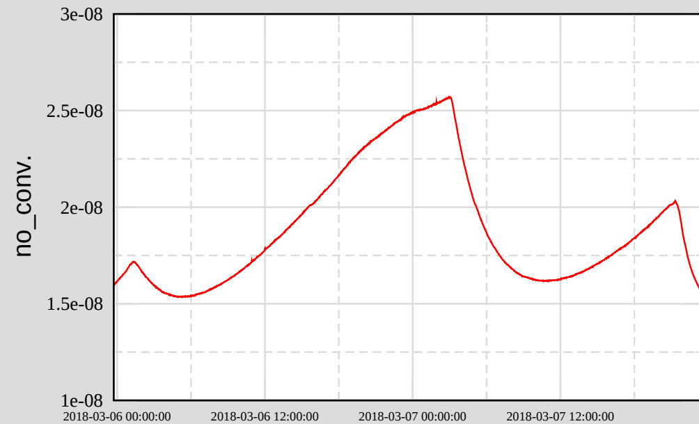
Ch 1: H0:VAC-MY_Y3_PT210B_PRESS_TORR
