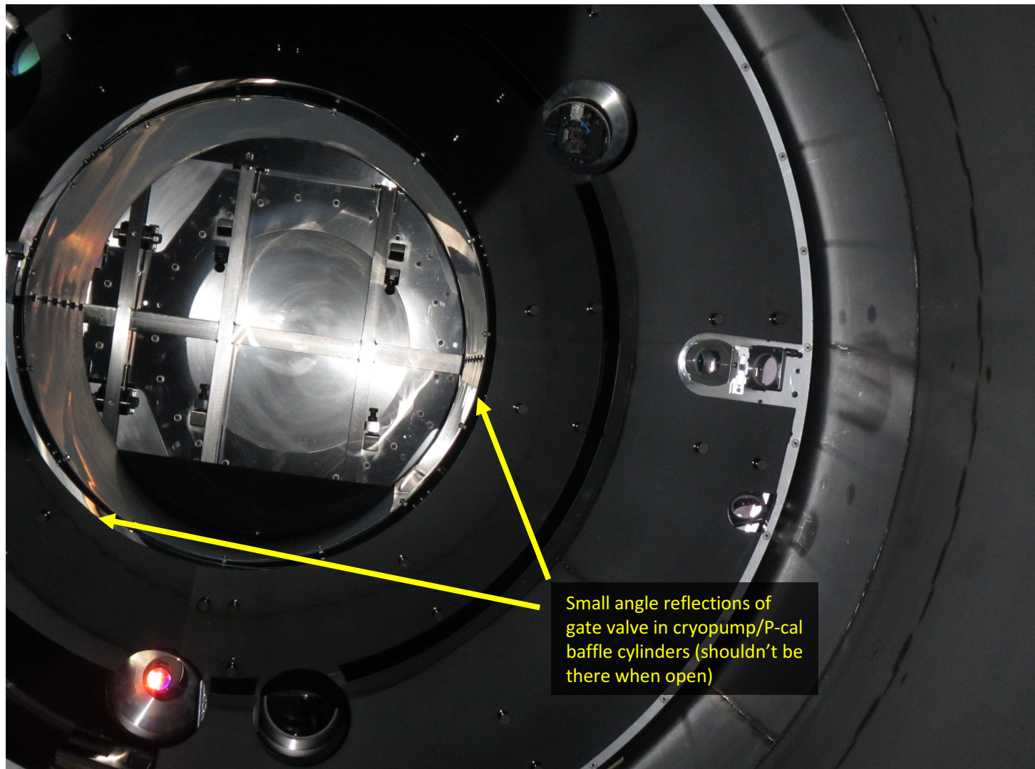
Figure 2. Close up of reflections in cryopump baffle and P-cal periscope baffle cylinders, thought to be reflections from gate valve
