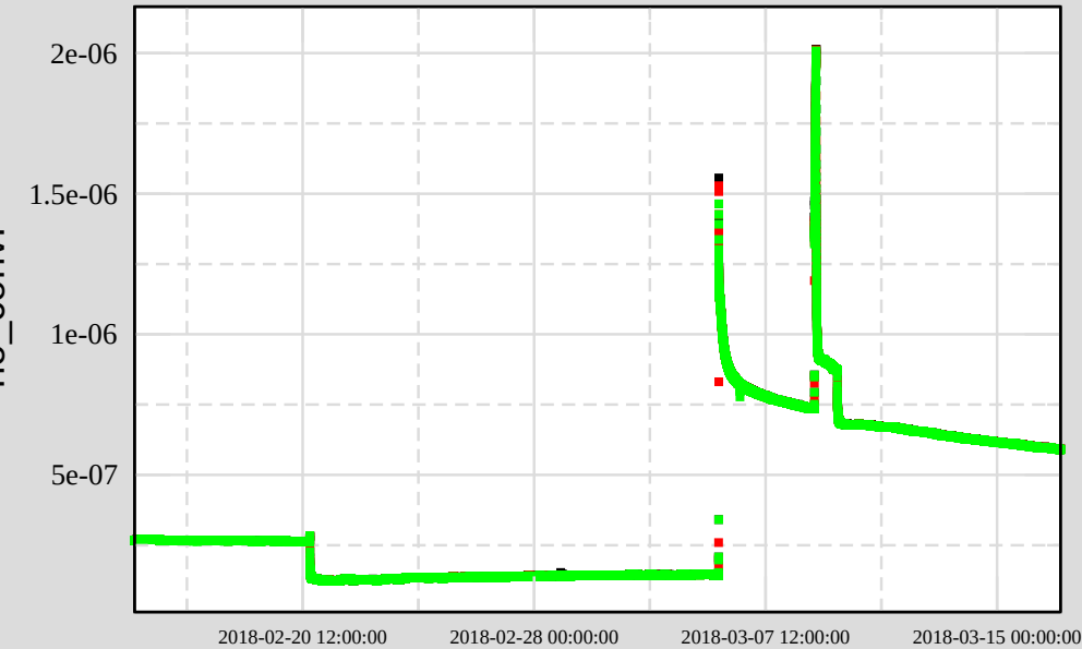
Ch 3: H0:VAC-LX_X2_PT170_MOD1_PRESS_TORR
