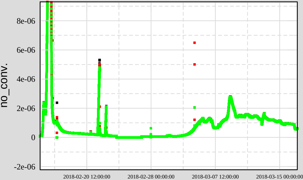
Ch 1: H0:VAC-MY_Y4_PT245B_PRESS_TORR
