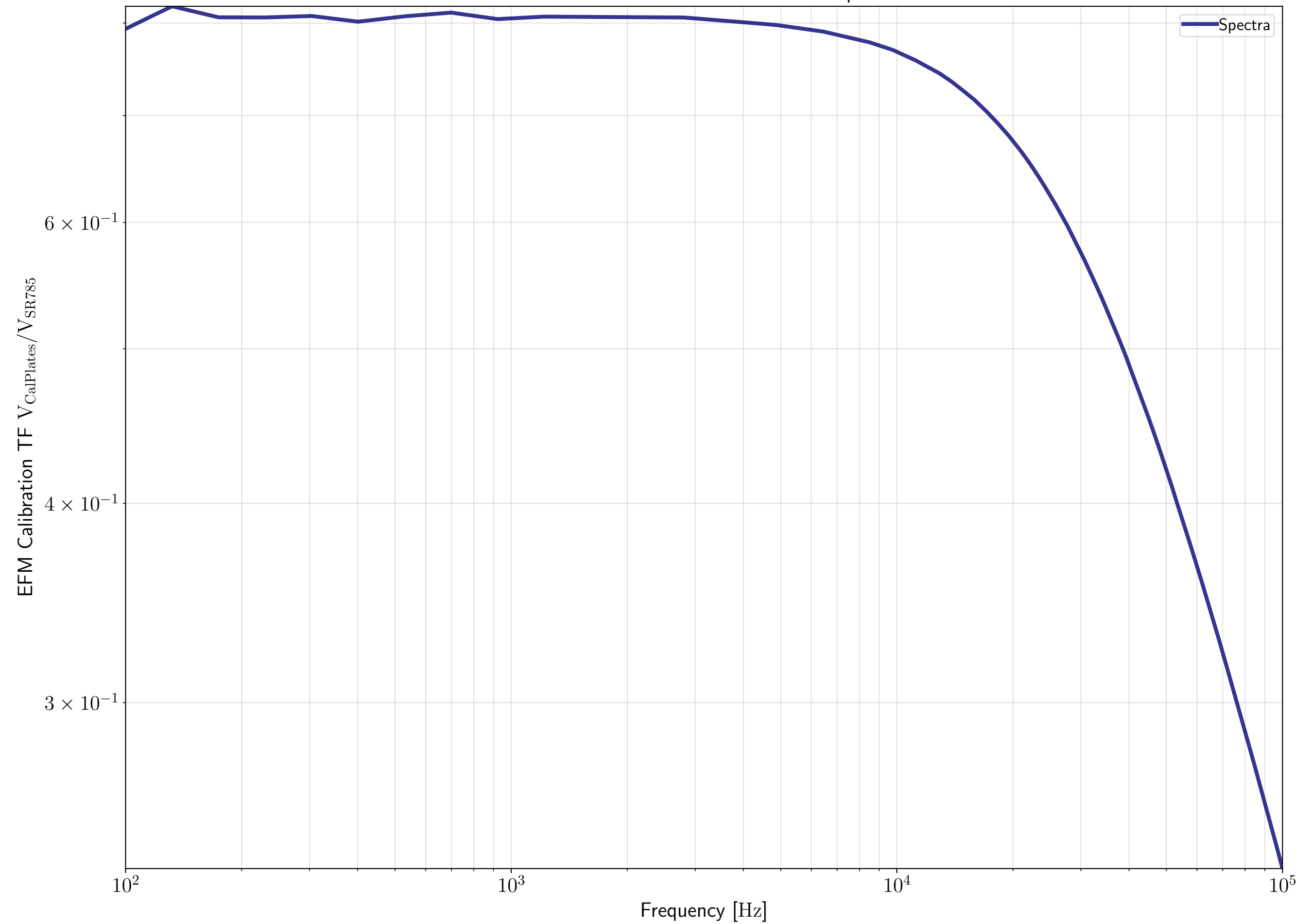
Electrometer Calibration TF - Positive Y - Apr-13-2018
