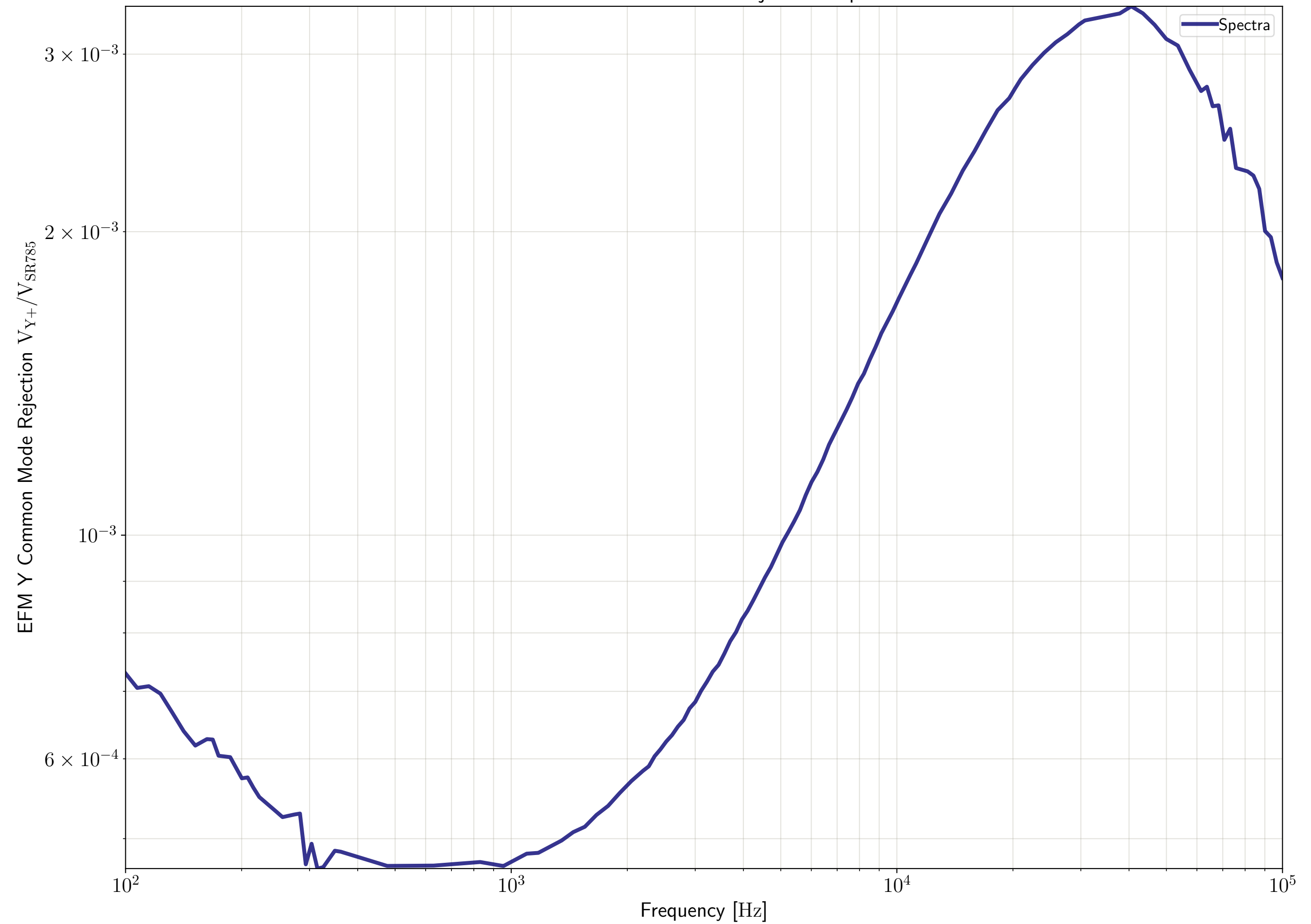
Electrometer Y Common Mode Rejection - Apr-13-2018
