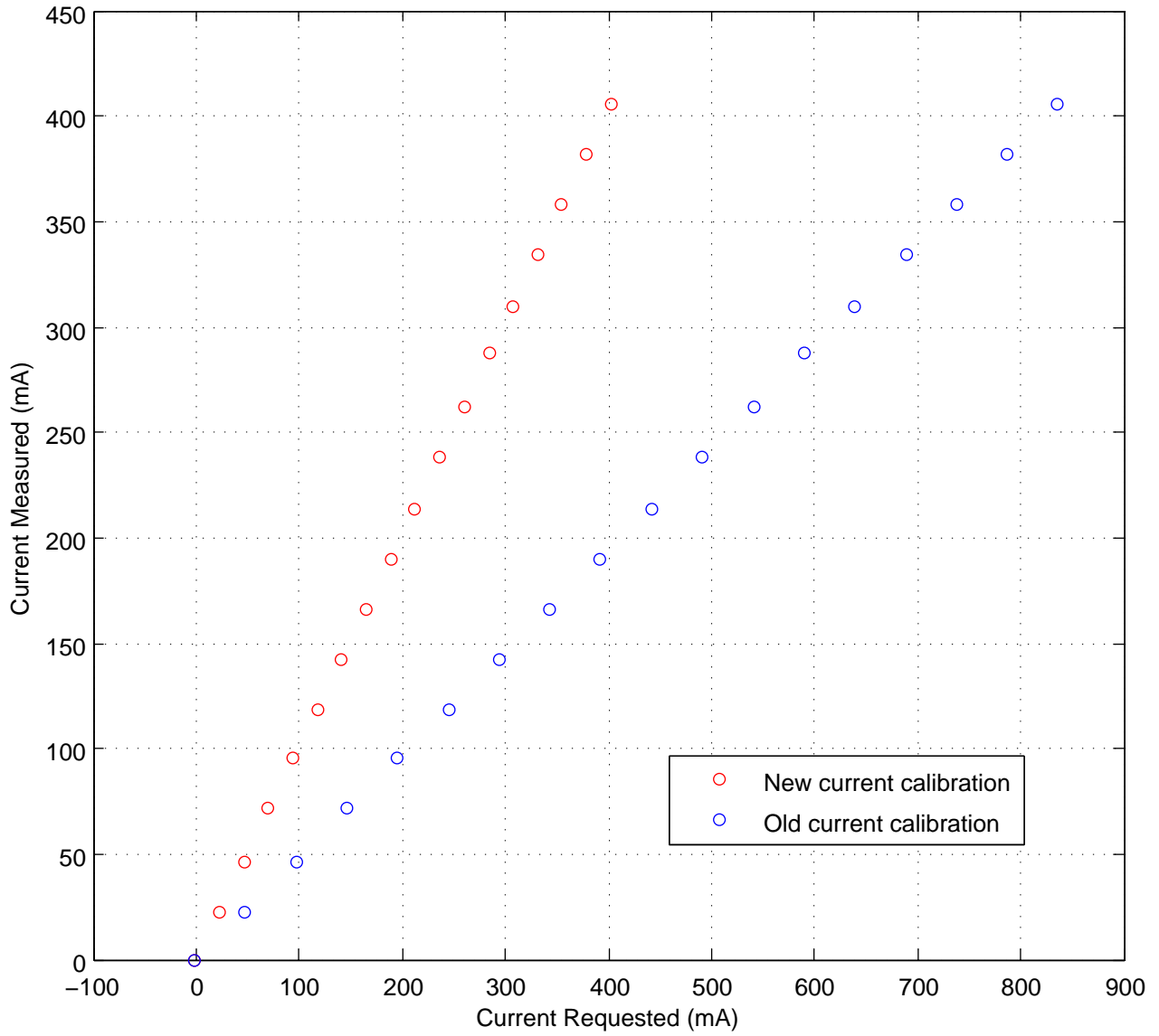
ETM Driver Calibration, 09-11-12
