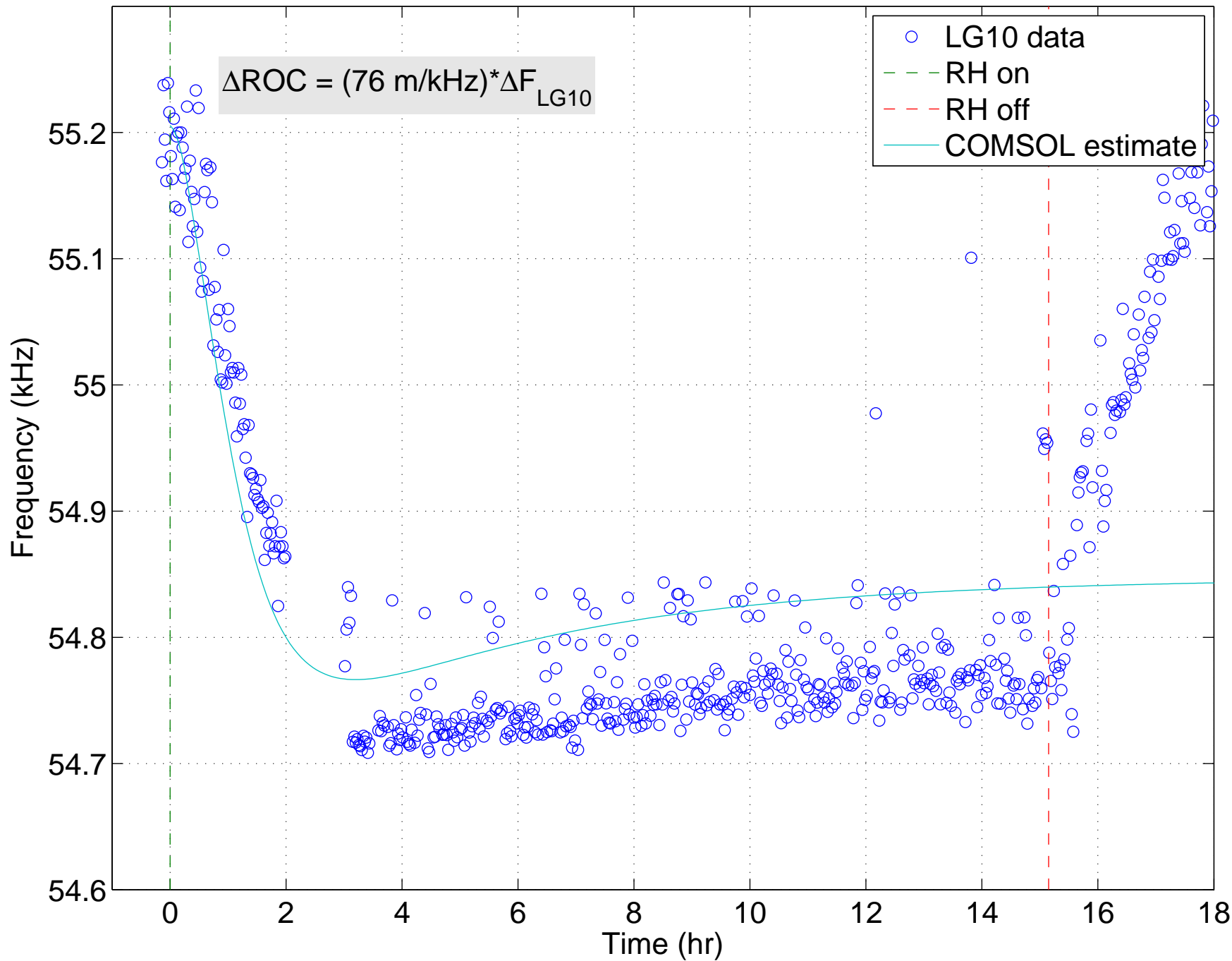
Lower sideband LG10 mode frequency vs time: 6.51W electrical power dissipated
