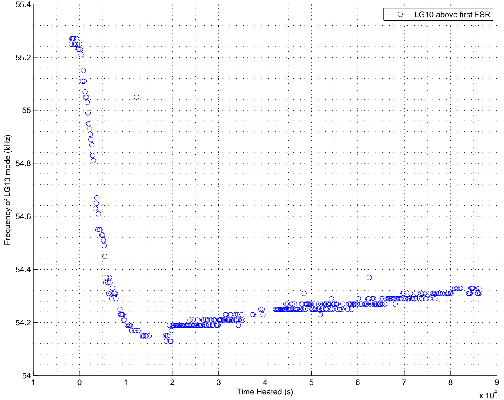
Shift of LG10 mode during ring heater operation – 13.2 W power dissipated
