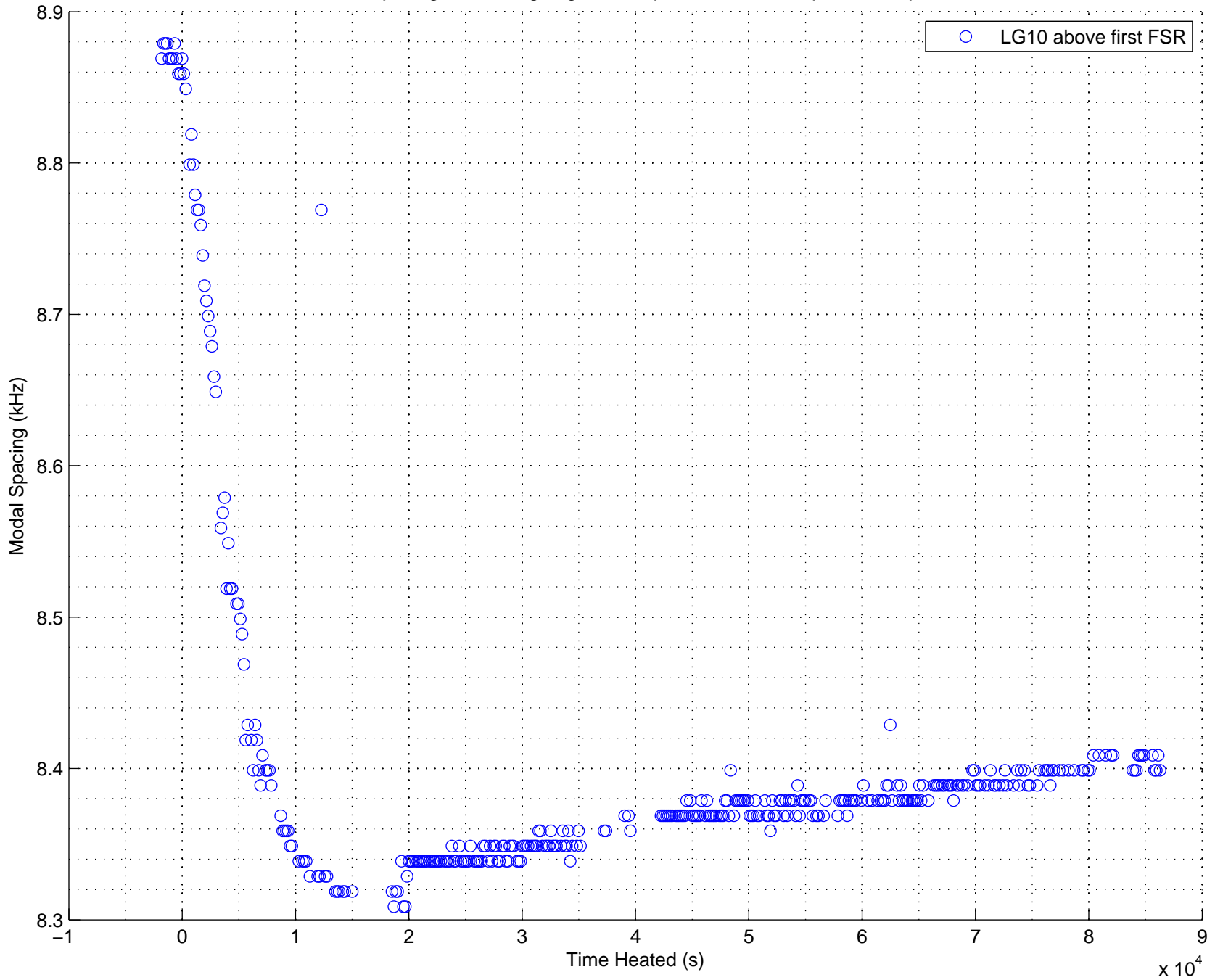
Modal spacing shift during ring heater operation – 13.2 W power dissipated
