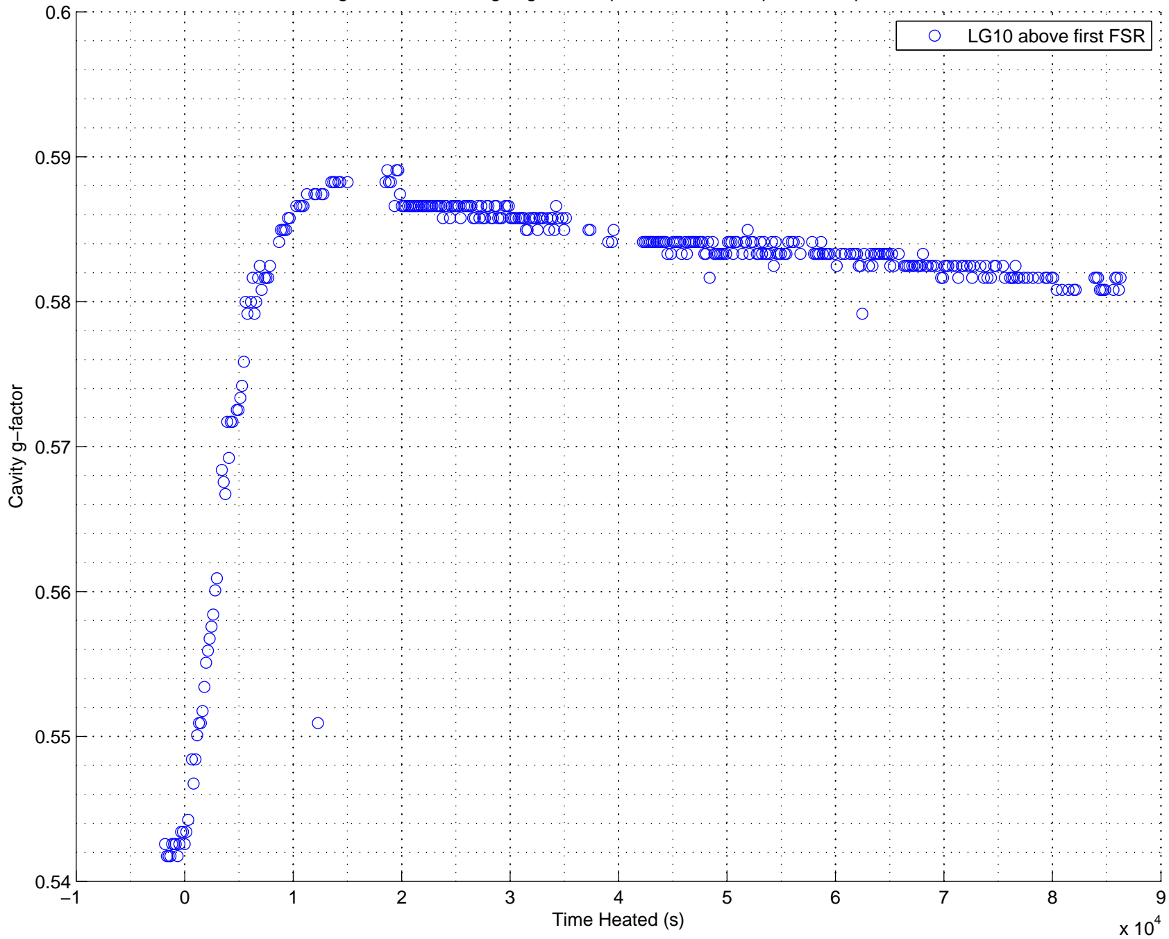
g-factor shift during ring heater operation – 13.2 W power dissipated
