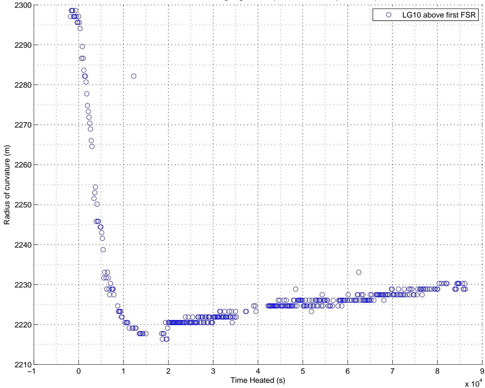
Radius of curvature shift during ring heater operation – 13.2 W power dissipated
